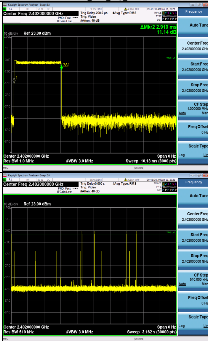
2DH5_Ant1_Hop_2402
