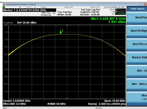
Channel 19 | 2 Mbps
