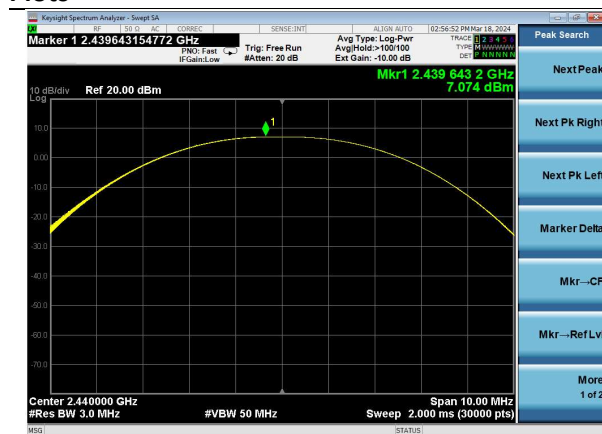
Channel 19 | 1 Mbps
