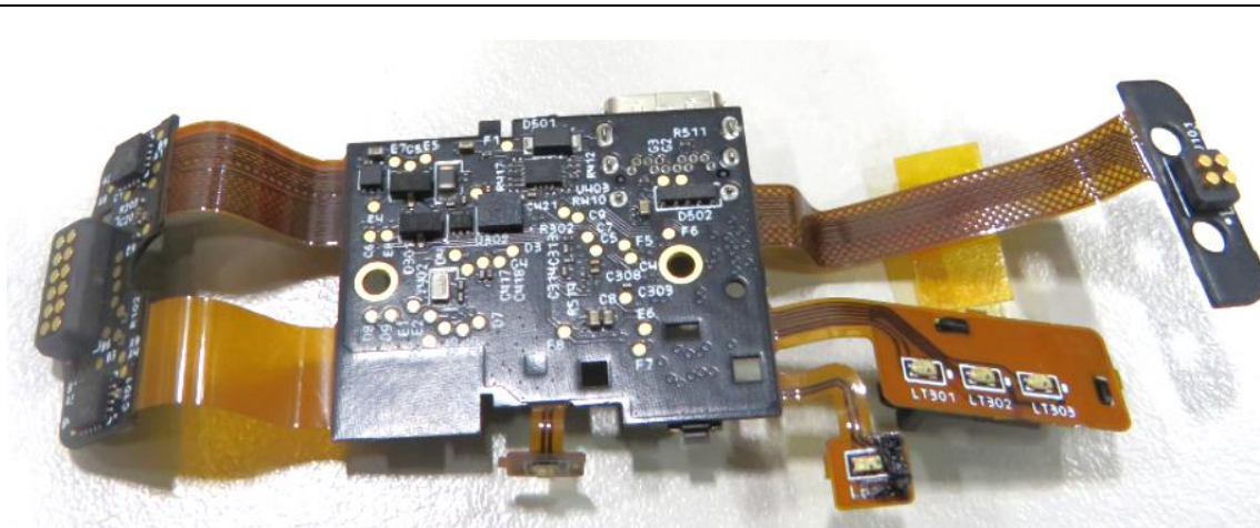
Photo #4 – Pod PCBs Bottom View
