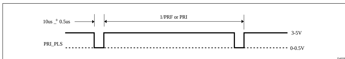
Figure 7: Modulator Clock, PRI_PLS
