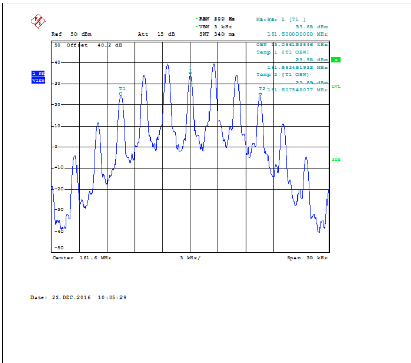
Plot 5.5.4.1.2. Occupied Bandwidth for 161.600 MHz, 25 kHz Channel Spacing, High Power, G3E
