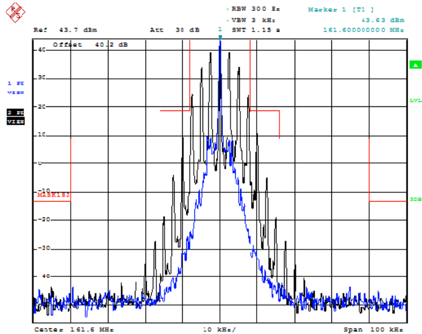
Plot 5.5.4.2.3. Emission Limitation for 161.600 MHz, 25 kHz Channel Spacing, High Power, G3E
