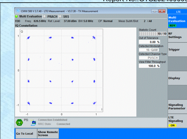
Band5-5MHz-16QAM-20425-25RB#0-PASS
