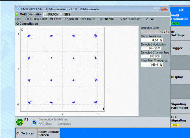
Band5-5MHz-16QAM-20525-25RB#0-PASS
