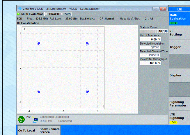
Band5-5MHz-QPSK-20525-25RB#0-PASS
