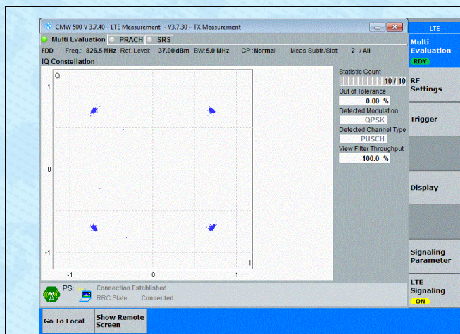
Band5-5MHz-QPSK-20425-25RB#0-PASS
