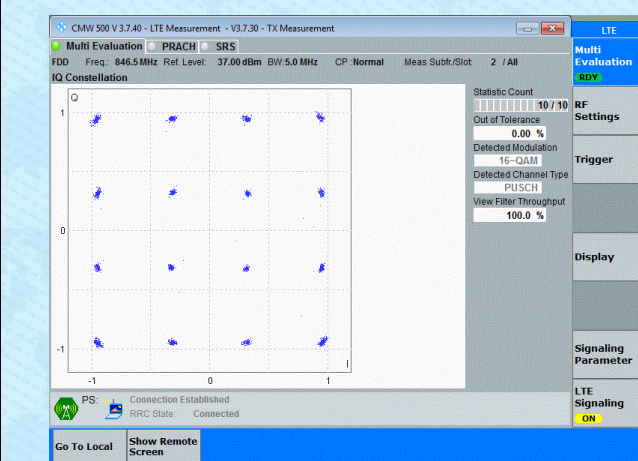
Band5-5MHz-16QAM-20625-25RB#0-PASS
