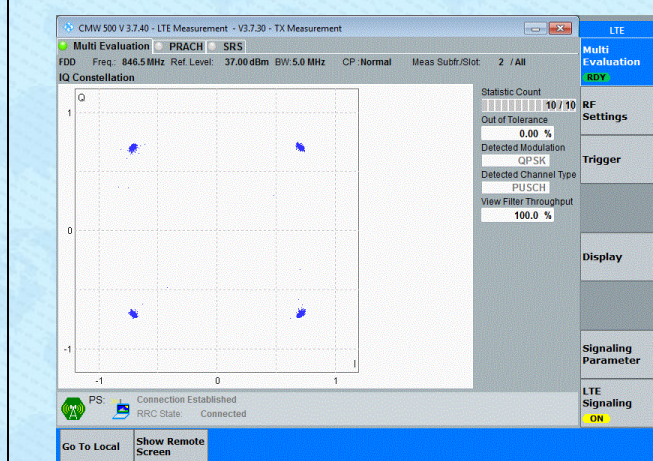
Band5-5MHz-QPSK-20625-25RB#0-PASS
