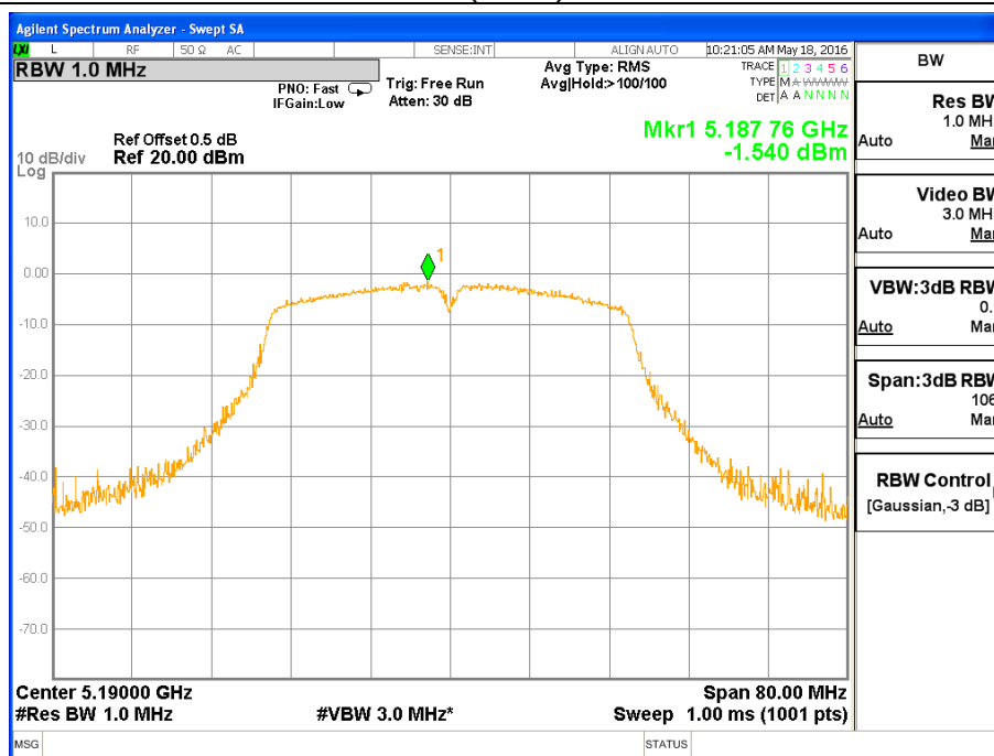
PSD 802.11n(HT40) Channel 38
