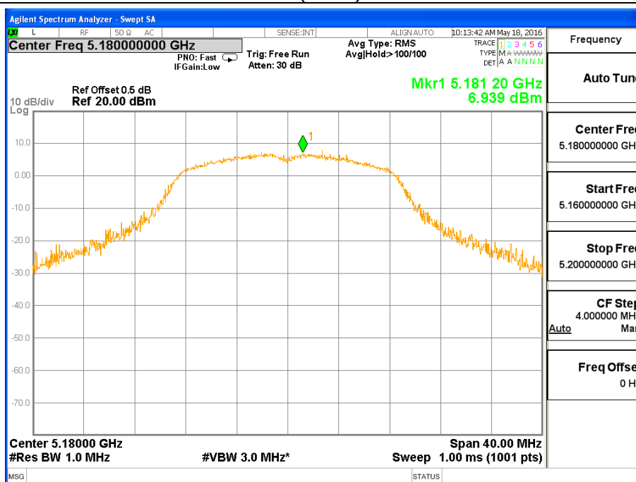
PSD 802.11n(HT20) Channel 36
