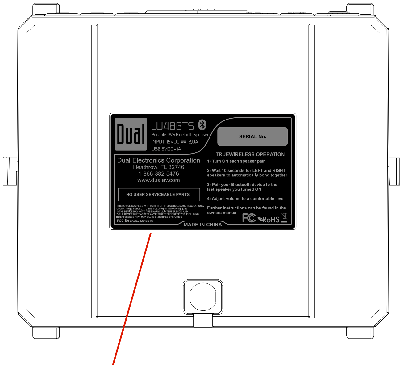
LU48BTS MODEL LABEL STICKER MATERIAL: 0.25mm PC SIZE: 80mm x 50mm PRINTED FROM THE BACKSIDE
