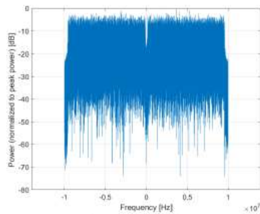
Frequency Domain
