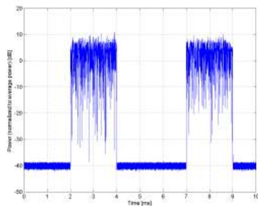
Time Domain
