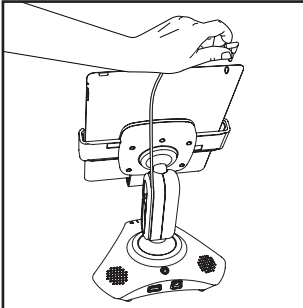
Connecting the Smart Device Cable
