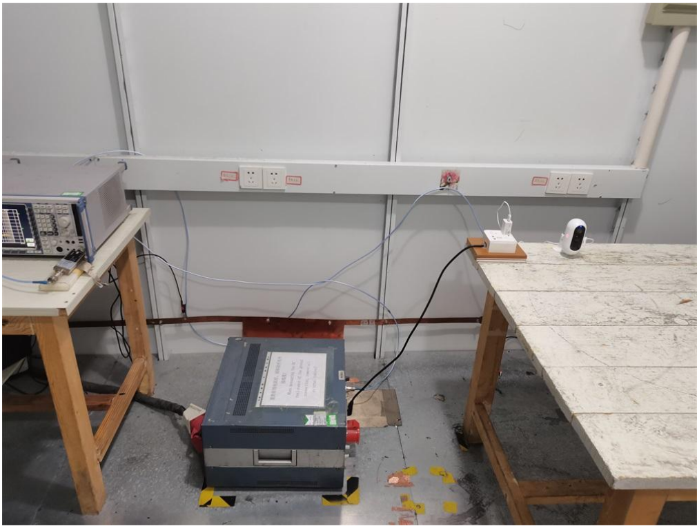
Conducted Emission
