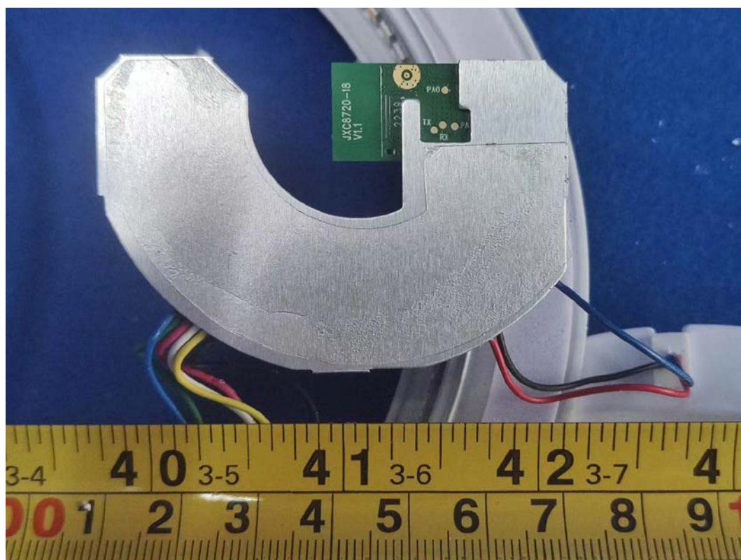
FIGURE 9 DOWNLIGHT (M/N: CFIXCNLR6SD) MAIN BOARD (SOLDERED SIDE)
