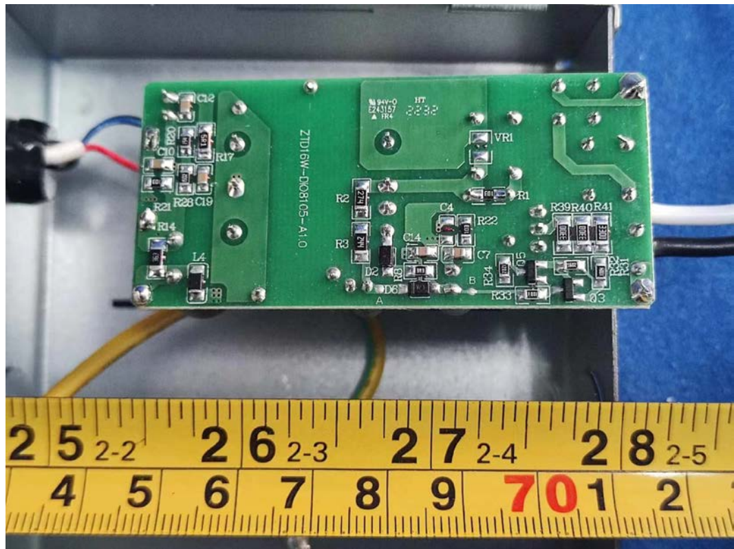
FIGURE 14 DOWNLIGHT (M/N: CFIXCNLR6S1) POWER BOARD (SOLDERED SIDE)
