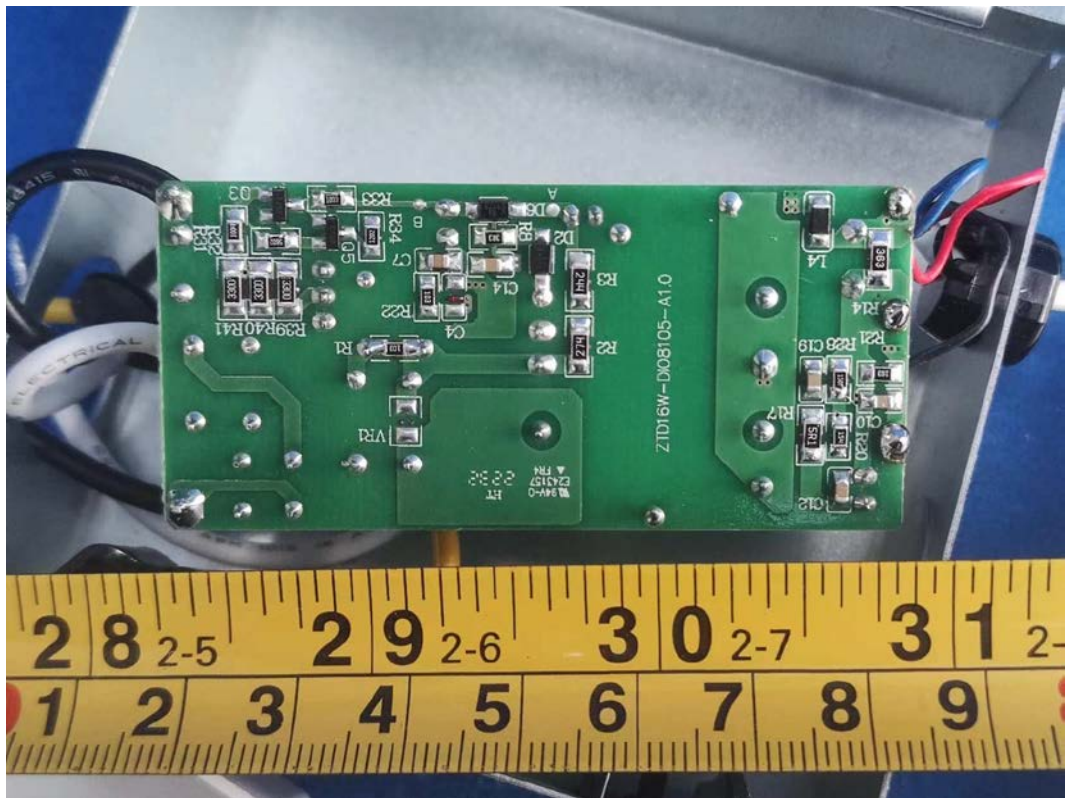
FIGURE 7 DOWNLIGHT (M/N: CFIXCNLR6SD) POWER BOARD (SOLDERED SIDE)
