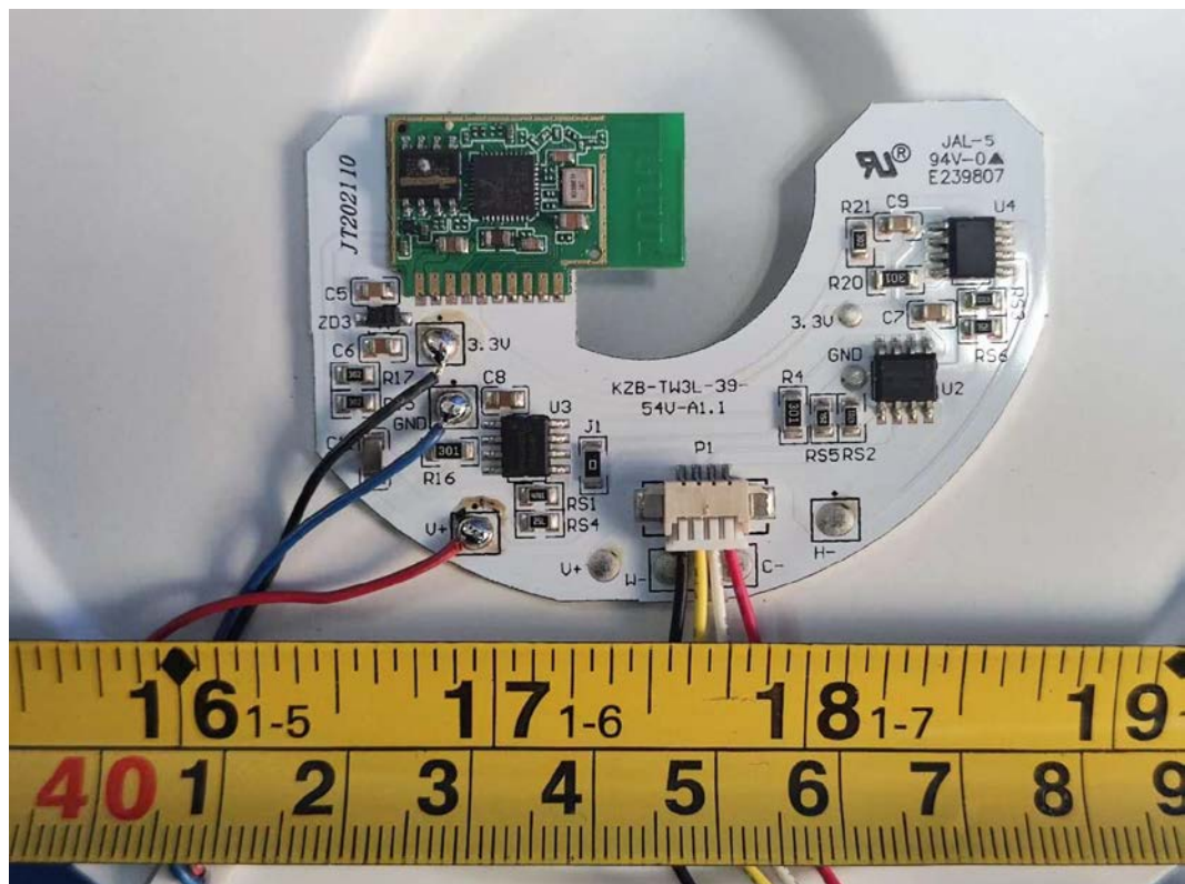
FIGURE 15 DOWNLIGHT (M/N: CFIXCNLR6S1) MAIN BOARD (COMPONENT SIDE)
