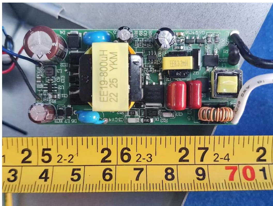
FIGURE 13 DOWNLIGHT (M/N: CFIXCNLR6S1) POWER BOARD (COMPONENT SIDE)
