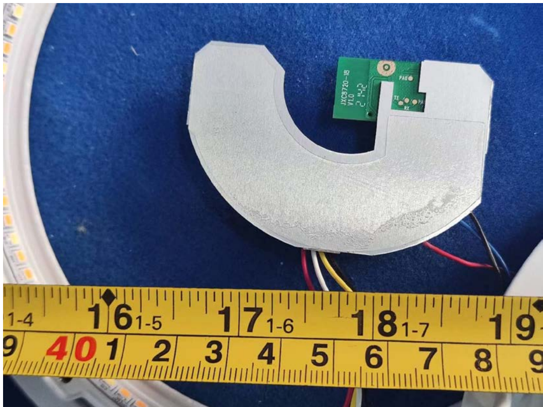
FIGURE 16 DOWNLIGHT (M/N: CFIXCNLR6S1) MAIN BOARD (SOLDERED SIDE)
