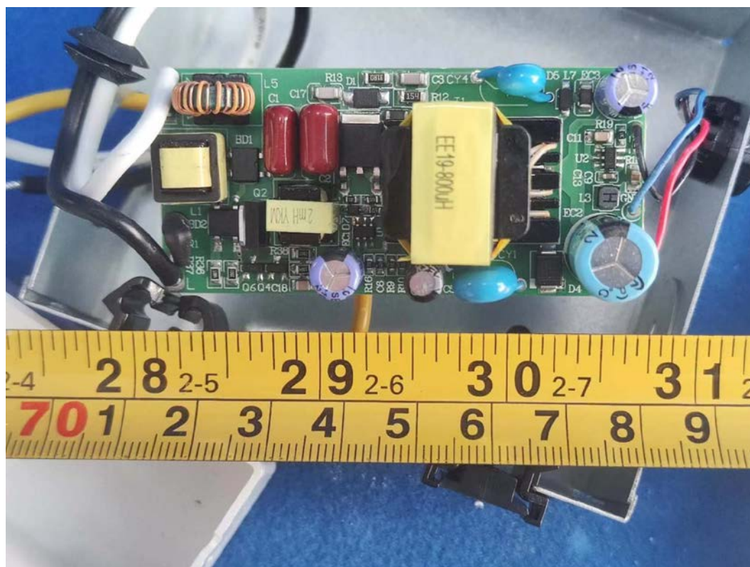
FIGURE 6 DOWNLIGHT (M/N: CFIXCNLR6SD) POWER BOARD (COMPONENT SIDE)
