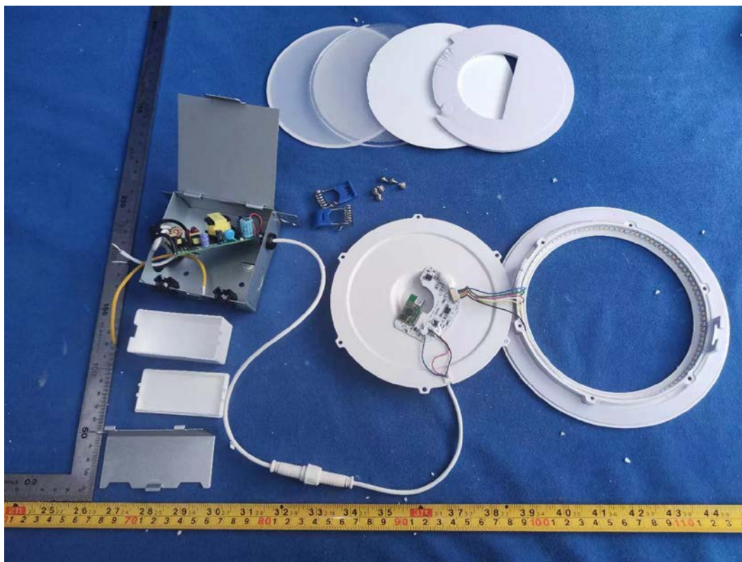
FIGURE 5 DOWNLIGHT (M/N: CFIXCNLR6SD) COVER REMOVED
