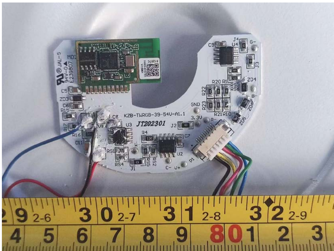
FIGURE 8 DOWNLIGHT (M/N: CFIXCNLR6SD) MAIN BOARD (COMPONENT SIDE)
