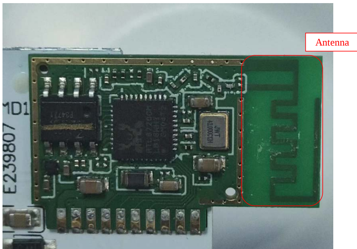
FIGURE 10 DOWNLIGHT (M/N: CFIXCNLR6SD) CHIP&CRYSTAL ON BOARD
