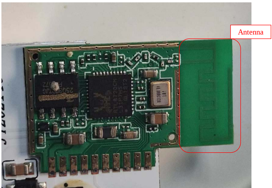
FIGURE 17 DOWNLIGHT (M/N: CFIXCNLR6S1) CHIP&CRYSTAL ON BOARD
