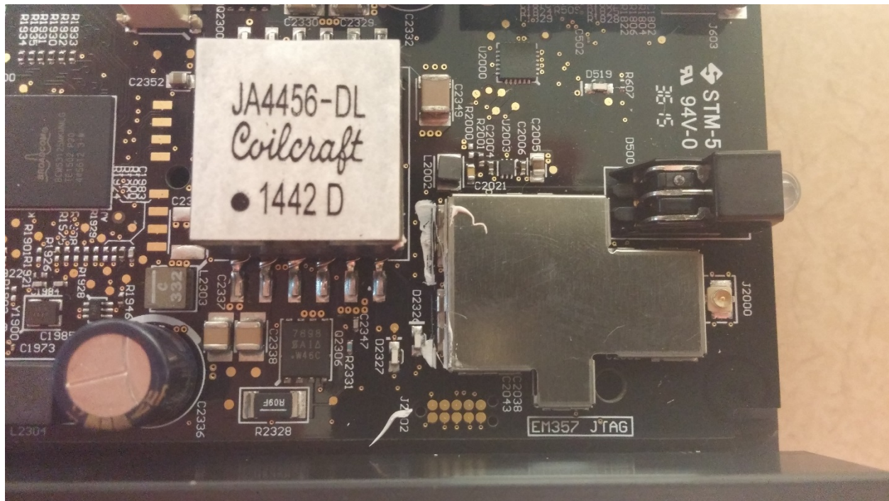
View of the 802.15.4 Transceiver Circuitry with RF Shield
