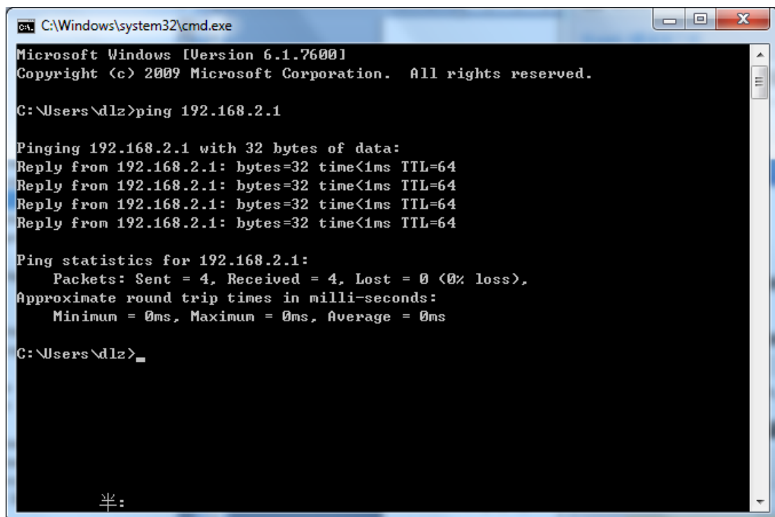
Figure 2-7 Command Prompt
