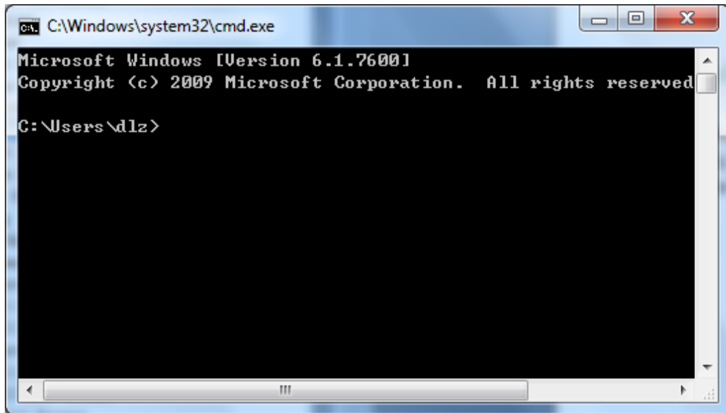
Figure 2-6 Run
