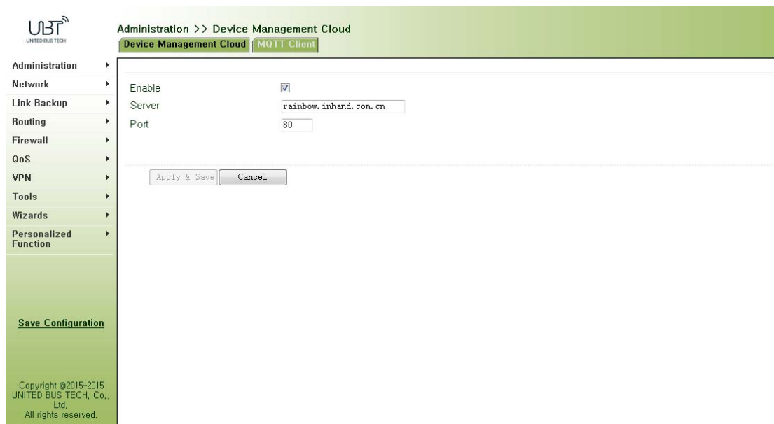
Figure 3-26 Cloud Platform
