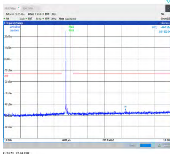
1-N66-PC3-15-40-H-1-DFT-PI2BPSK-Inner_1RB_Lef t-1@1-1000-3000-Ant0--45.49--13-PASS
