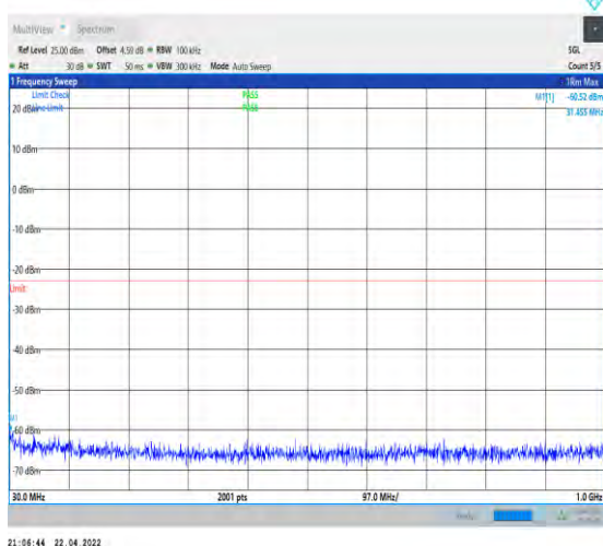
1-N66-PC3-15-40-H-1-DFT-PI2BPSK-Inner_1RB_Le ft-1@1-30-1000-Ant0--60.52--23-PASS
