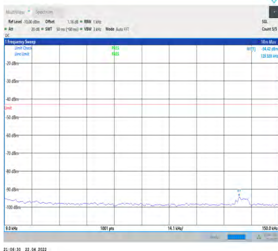
1-N66-PC3-15-40-H-1-DFT-PI2BPSK-Inner_1RB_Le ft-1@1-0.009-0.15-Ant0--94.42--43-PASS
