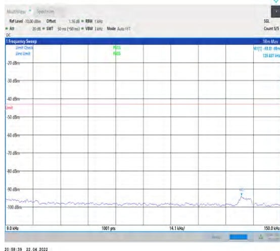
1-N66-PC3-15-40-L-1-DFT-PI2BPSK-Inner_1RB_Le ft-1@1-0.009-0.15-Ant0--93.81--43-PASS
