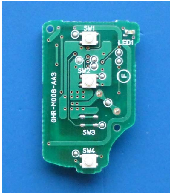
Figure 7.7 PCB (front view)
