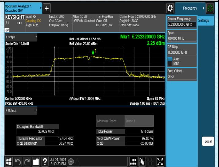
11AC40SISO-Ant1-5230
