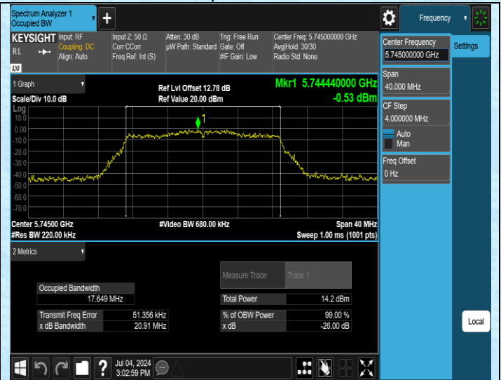
11AC20SISO-Ant1-5745
