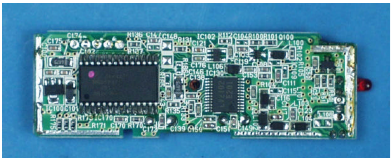
RF Board, Side 1 w/o Shield
