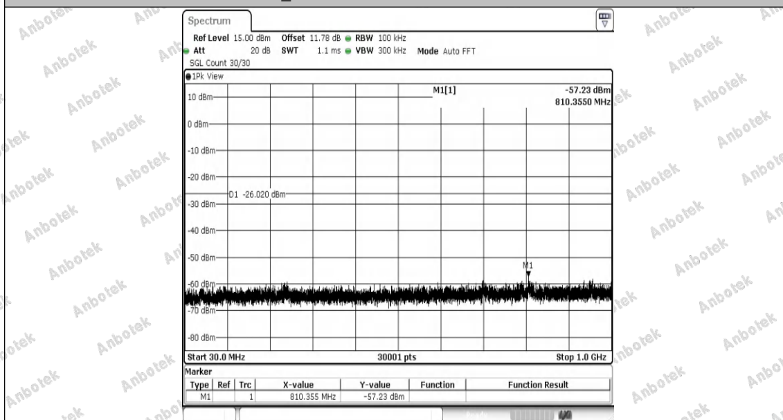
BLE_2M-Ant1-2440-0~Reference-PASS
