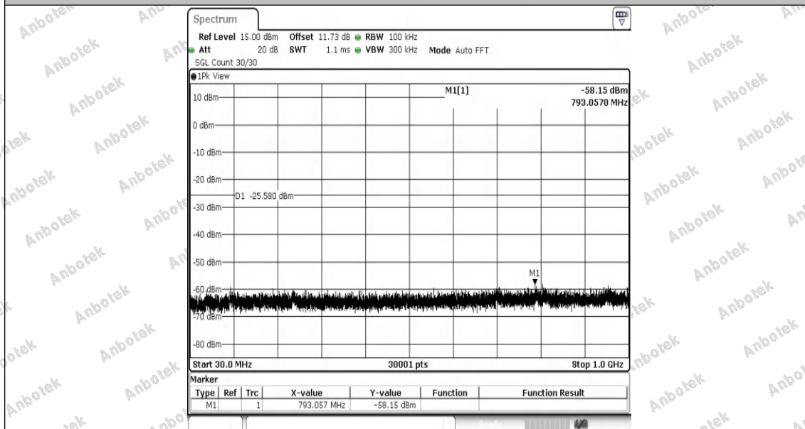
BLE_1M-Ant1-2480-30~1000-PASS
