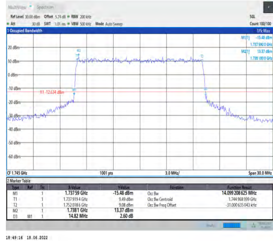
1-N66--15-15-M-7-CP-16QAM-Outer_Full-79@0-Ant1 -14.099-14.820≤15-PASS
