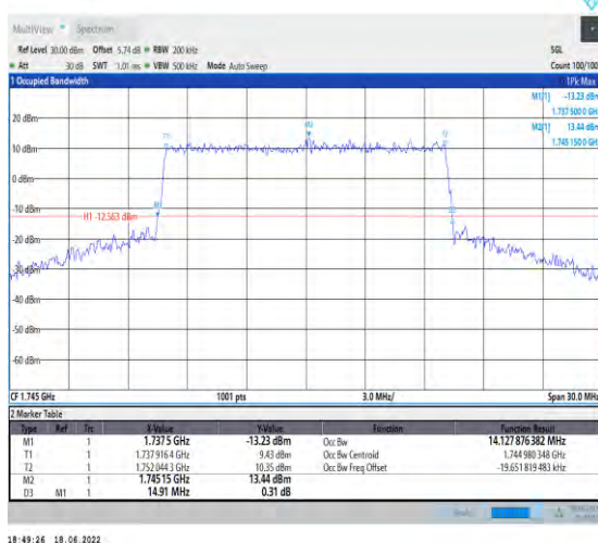
1-N66--15-15-M-8-CP-64QAM-Outer_Full-79@0-Ant1 1-14.128-14.910≤15-PASS
