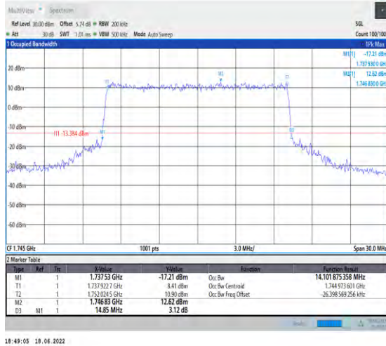
1-N66--15-15-M-6-CP-QPSK-Outer_Full-79@0-Ant1 -14.102-14.850≤15-PASS
