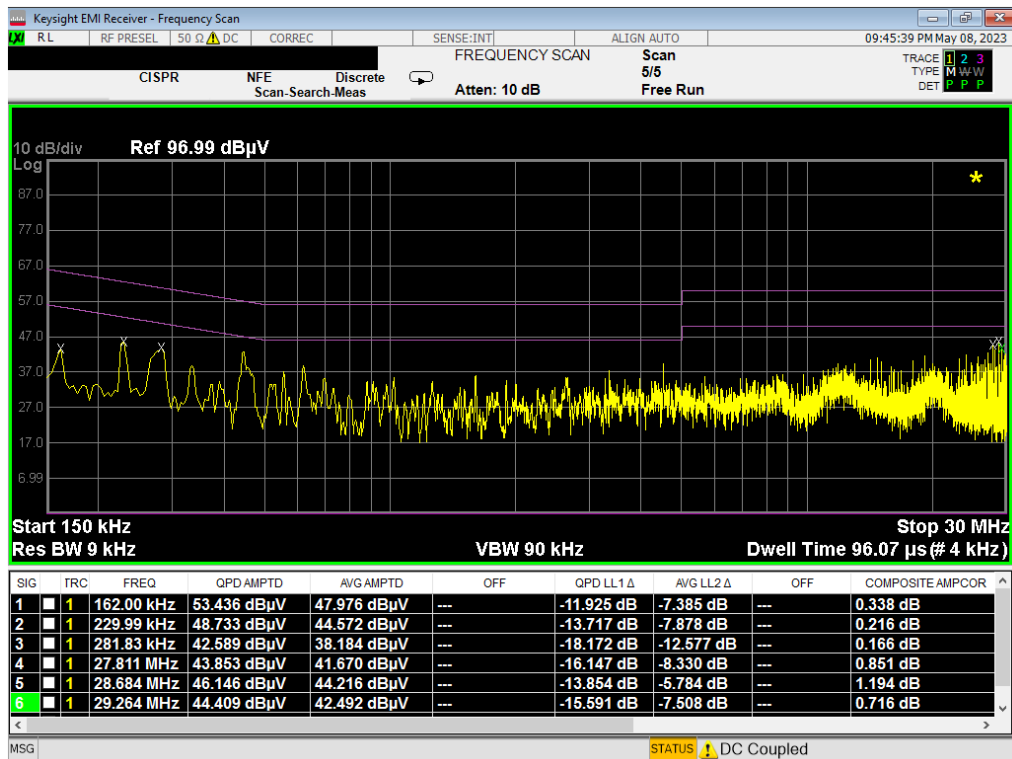
Plot 7-6. Line-Conducted Test Plot (N) - Device to Device
