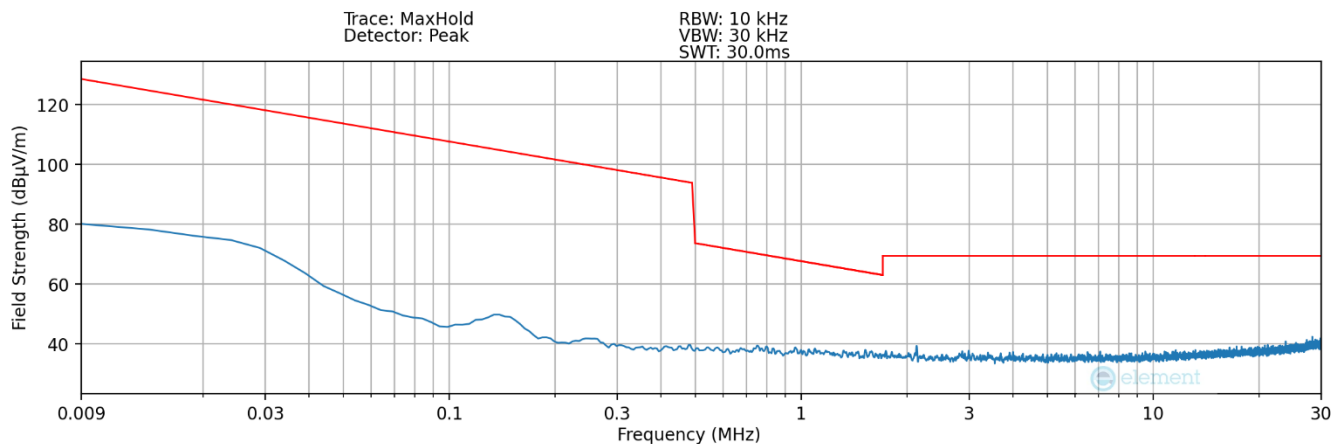
Plot 7-4. Radiated Spurious Plot 9kHz – 30MHz (Pol. Z – Device to Device WPT)
