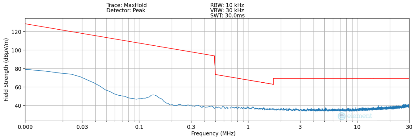
Plot 7-3. Radiated Spurious Plot 9kHz – 30MHz (Pol. Y – Device to Device WPT)
