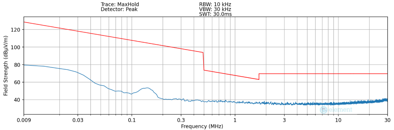
Plot 7-2. Radiated Spurious Plot 9kHz – 30MHz (Pol. X – Device to Device WPT)
