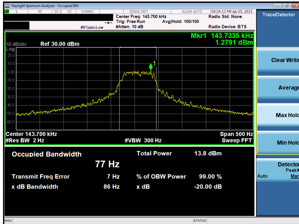
Plot 7-1. Occupied Bandwidth Measurement
