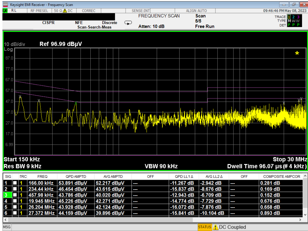
Plot 7-5. Line-Conducted Test Plot (L1) - Device to Device
