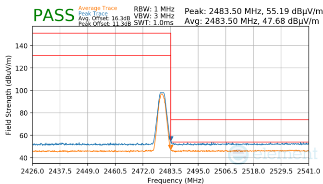
Plot 7-51. Radiated Restricted Upper Band Edge Measurement (Average & Peak)
