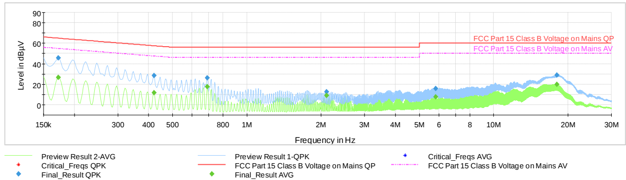
Plot 7-53. Line Conducted Plot with Bluetooth LE (N)
