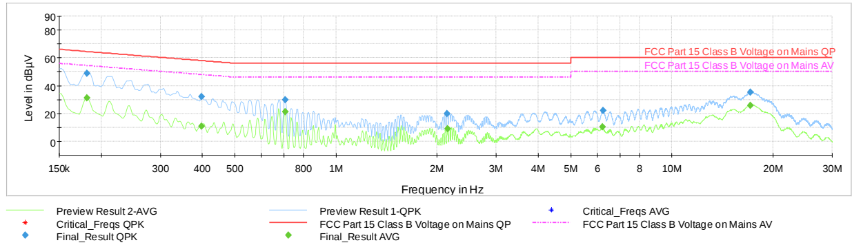
Plot 7-52. Line Conducted Plot with Bluetooth LE (L1)
