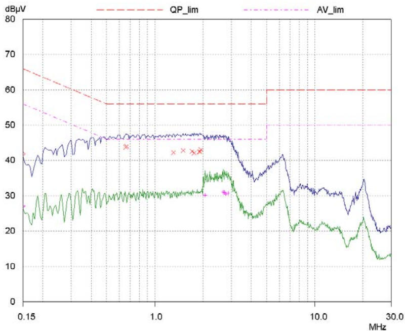
Picture 22: AC power line emissions, line L.
