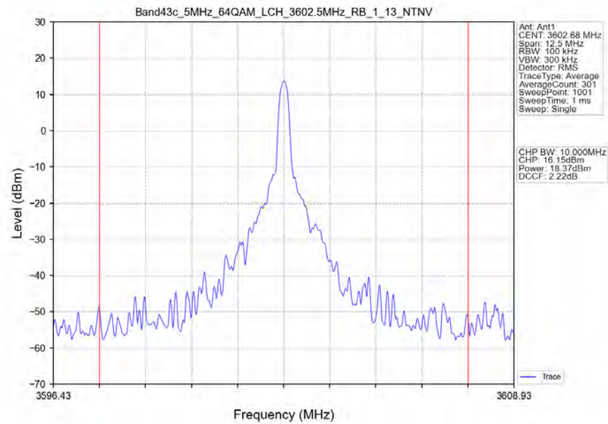
Band43c_5MHz_64QAM_LCH_3602.5MHz_RB_1_13_NTNV
