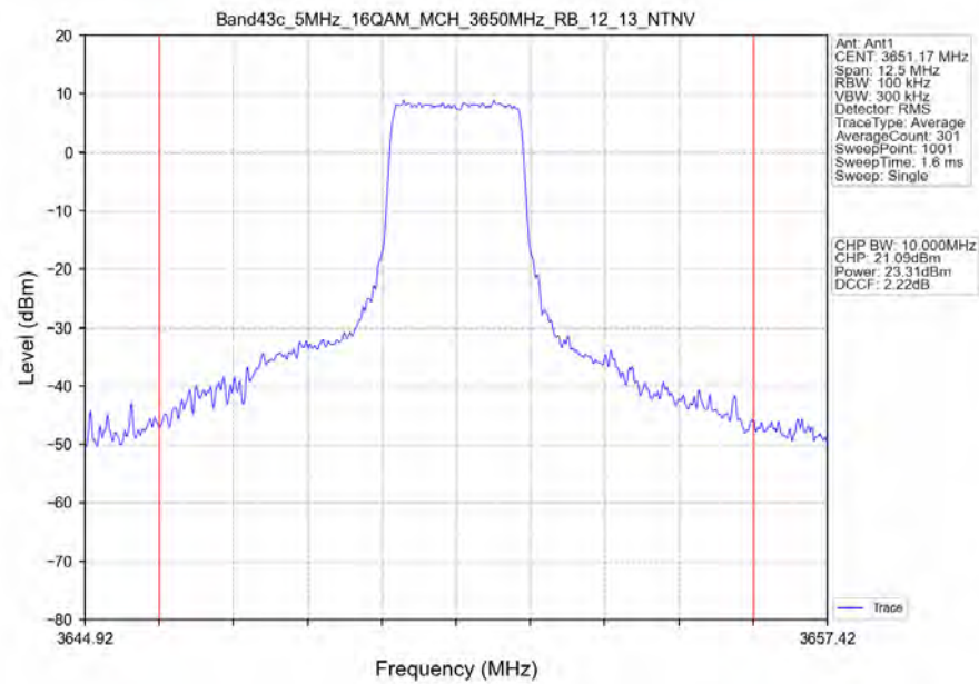
Band43c_5MHz_16QAM_MCH_3650MHz_RB_12_13_NTNV
