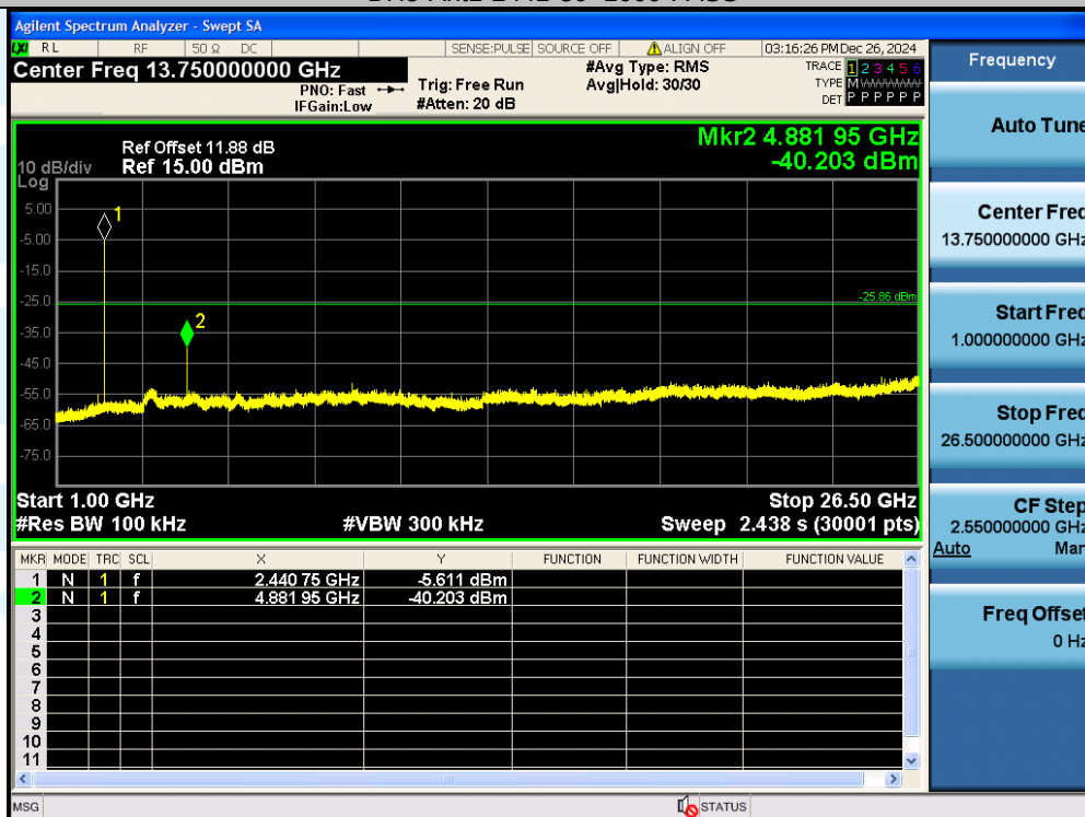
DH5-Ant1-2441-1000~26500-PASS
