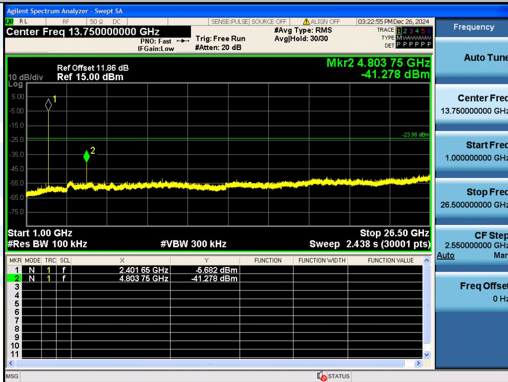
2DH5-Ant1-2402-1000~26500-PASS
