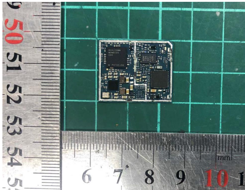
Photo 33 - Quectel BG95-M3
