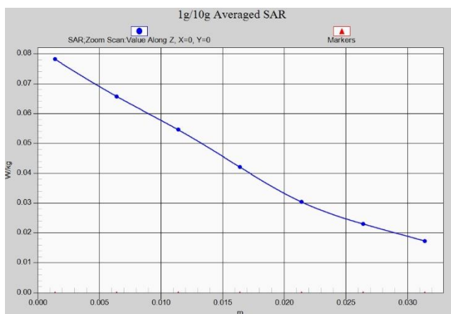
Fig. 4-1 Z-Scan at power reference point (GSM 1900)
