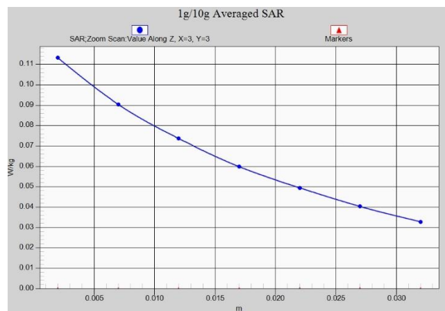
Fig. 21-1 Z-Scan at power reference point (LTE Band13)
