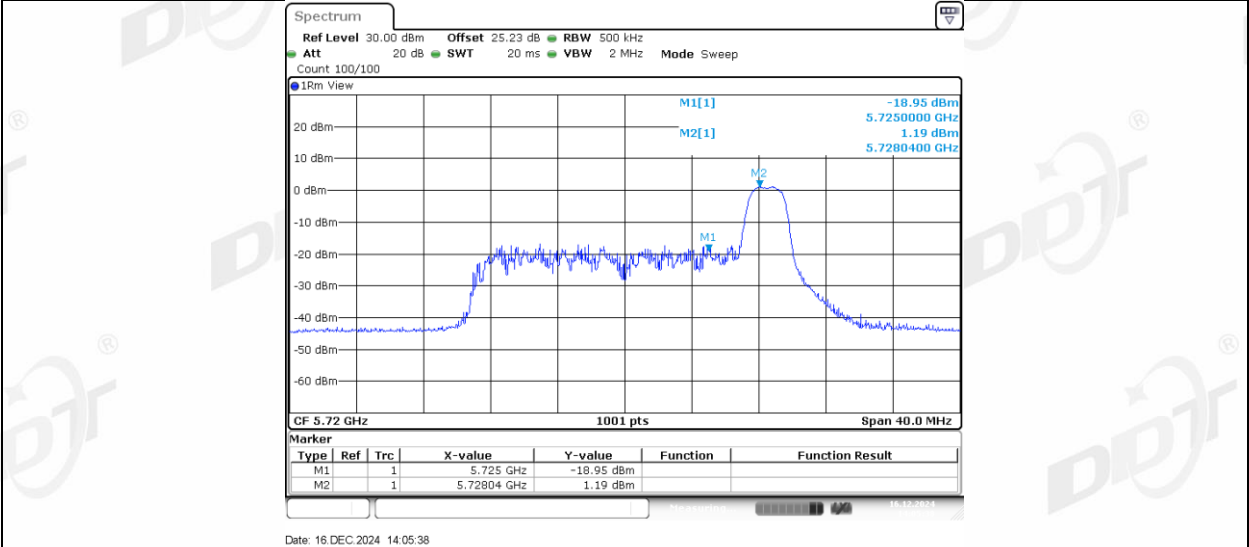
11AX20MIMO Ant1 5720 UNII-3 52Tone RU37
