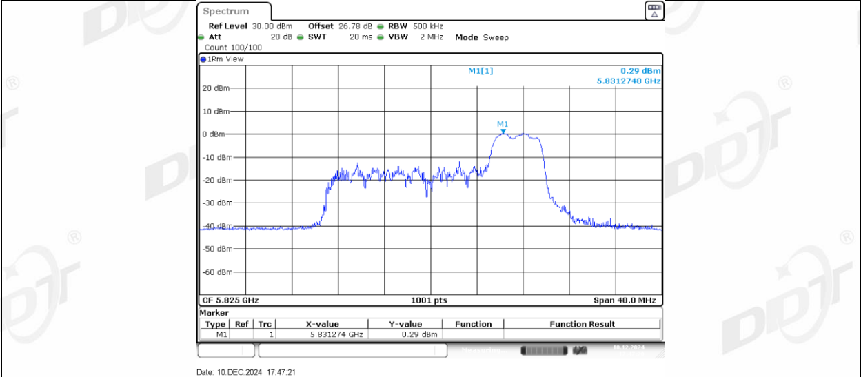
11AX20MIMO Ant1 5825_106Tone RU53
