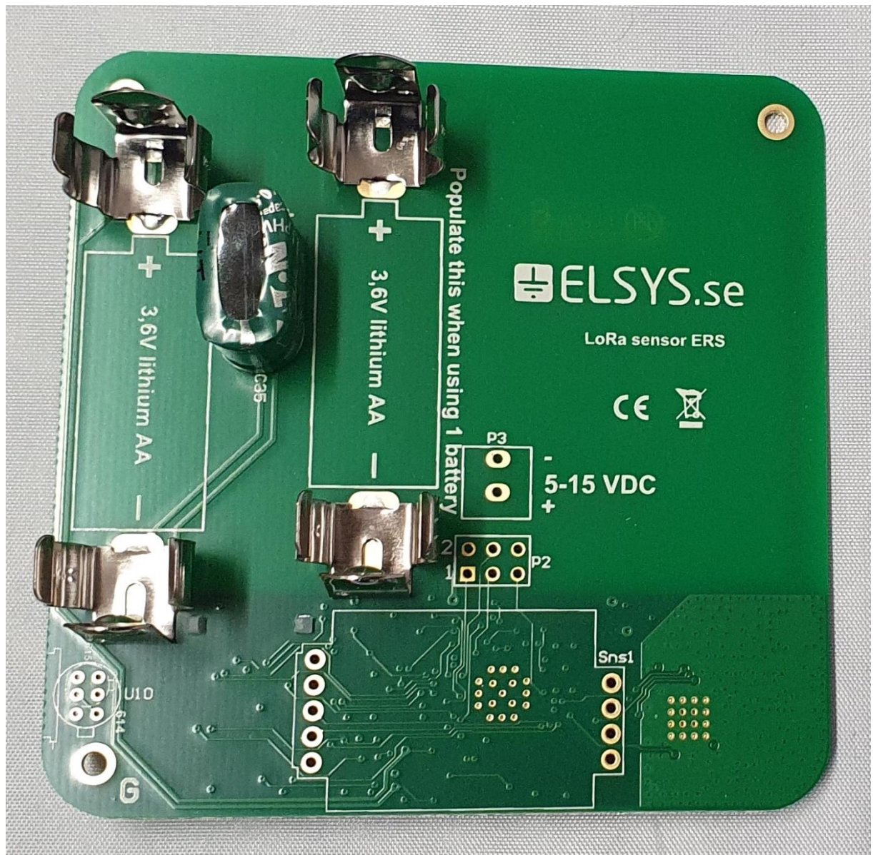
PCB-back
