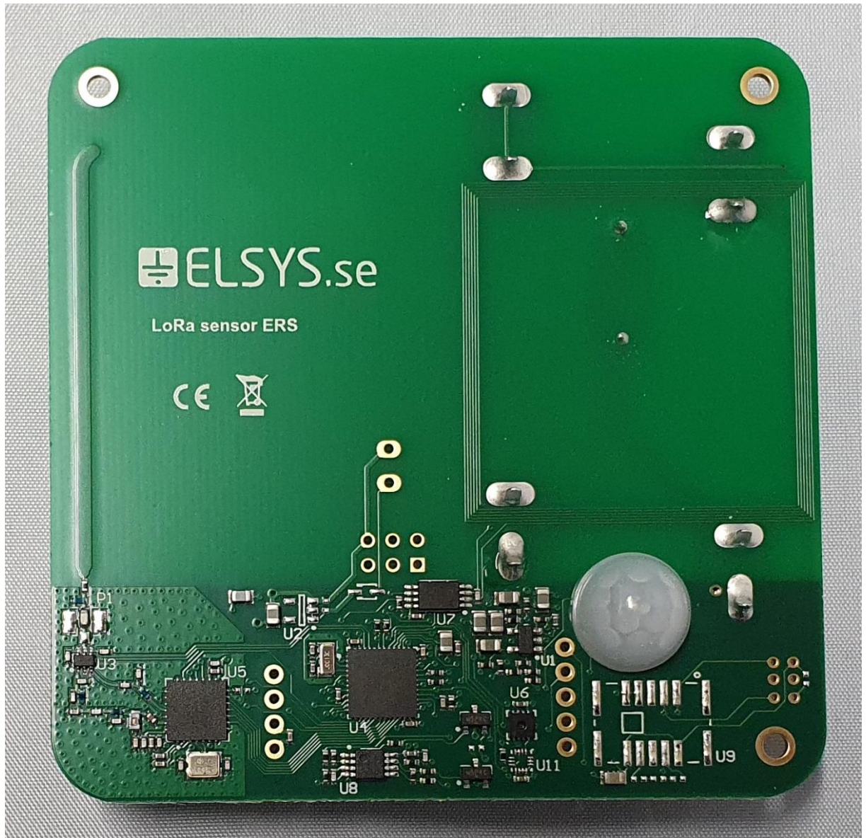
PCB-front
