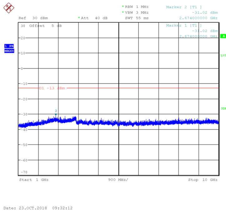
Fig.62 Channel 251: 1GHz~10GHz
