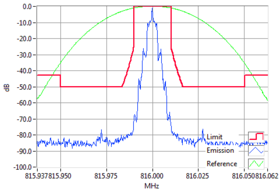
FFSK2400 816.000MHz Mask G 1W RBW=300Hz, VBW=3000Hz, Detector Mode=Peak Result=Pass
