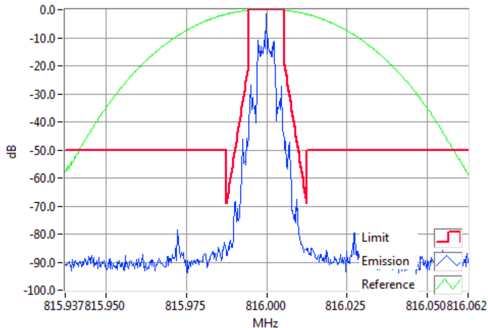
FFSK2400 816.000MHz Mask D 1W RBW=100Hz, VBW=1000Hz, Detector Mode=Peak Result=Pass
