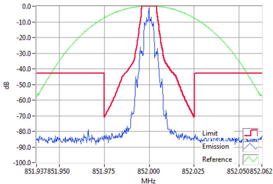
FFSK2400 852.000MHz Mask H 1W RBW=300Hz, VBW=3000Hz, Detector Mode=Peak Result=Pass
