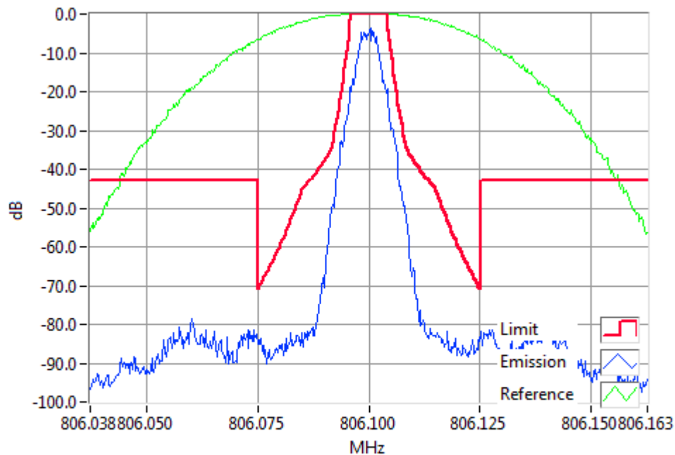
P25I 806.1000MHz Mask H 1W RBW=300Hz, VBW=3000Hz, Detector Mode=Peak Result=Pass
