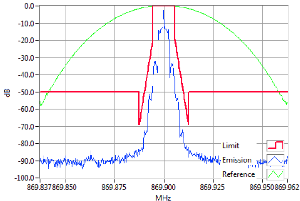
FFSK2400 869.9000MHz Mask D 1W RBW=100Hz, VBW=1000Hz, Detector Mode=Peak Result=Pass
