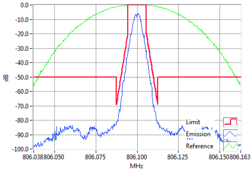
P25I 806.1000MHz Mask D 1W RBW=100Hz, VBW=1000Hz, Detector Mode=Peak Result=Pass
