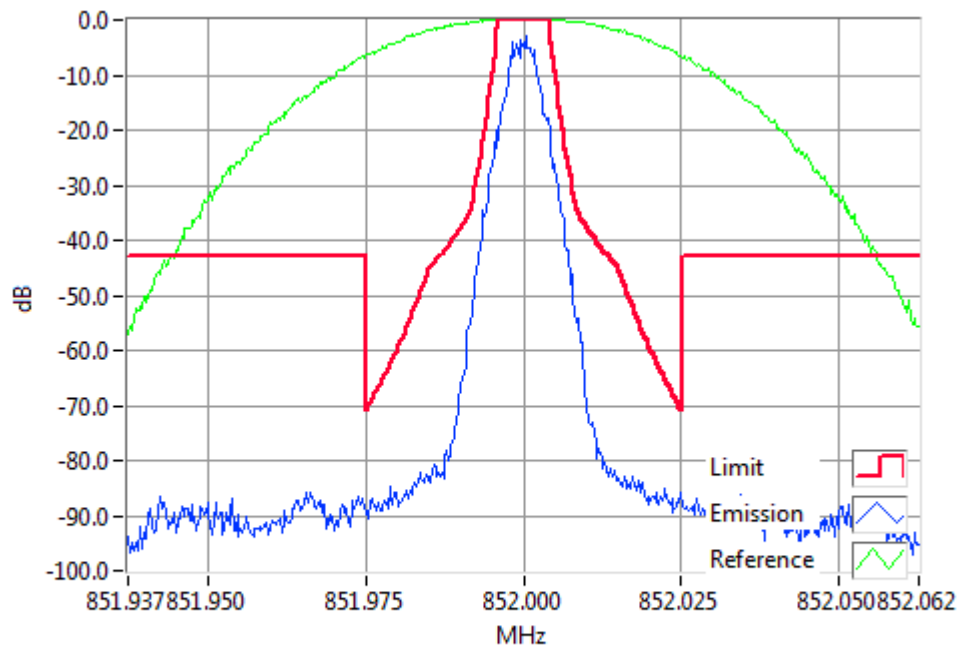
P25I 852.0000MHz Mask H 1W RBW=300Hz, VBW=3000Hz, Detector Mode=Peak Result=Pass
