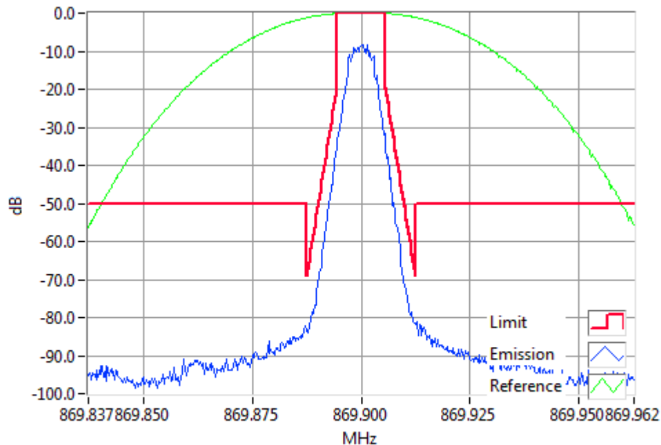
P25II 869.9000MHz Mask D 1W RBW=100Hz, VBW=1000Hz, Detector Mode=Peak Result=Pass
