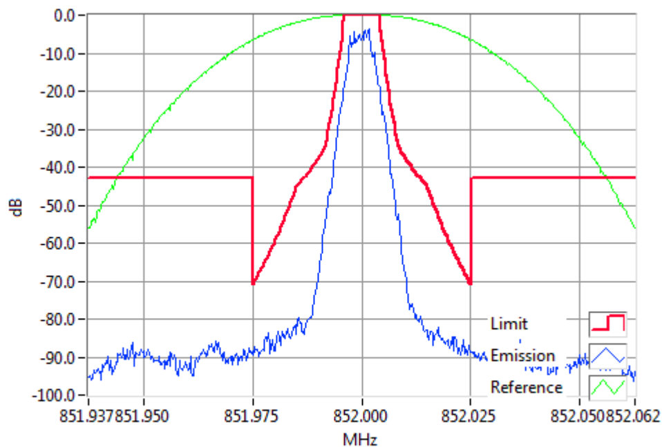
P25II 852.0000MHz Mask H 1W RBW=300Hz, VBW=3000Hz, Detector Mode=Peak Result=Pass
