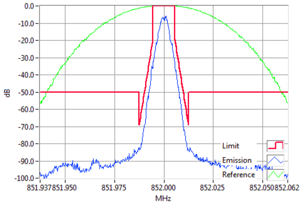
P25I 852.0000MHz Mask D 1W RBW=100Hz, VBW=1000Hz, Detector Mode=Peak Result=Pass
