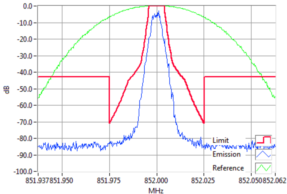
DMR 852.0000MHz Mask H 1W RBW=300Hz, VBW=3000Hz, Detector Mode=Peak Result=Pass
