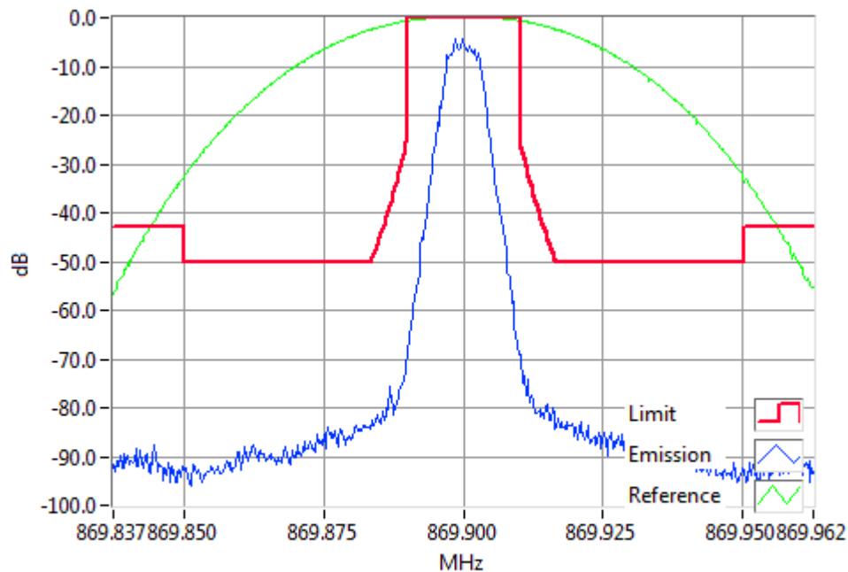
P25II 869.9000MHz Mask G 1W RBW=300Hz, VBW=3000Hz, Detector Mode=Peak Result=Pass
