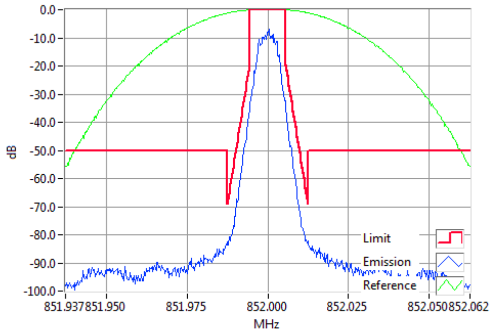
P25II 852.0000MHz Mask D 1W RBW=100Hz, VBW=1000Hz, Detector Mode=Peak Result=Pass
