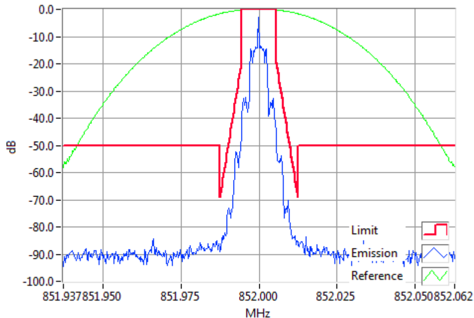
FFSK2400 852.000MHz Mask D 1W RBW=100Hz, VBW=1000Hz, Detector Mode=Peak Result=Pass
