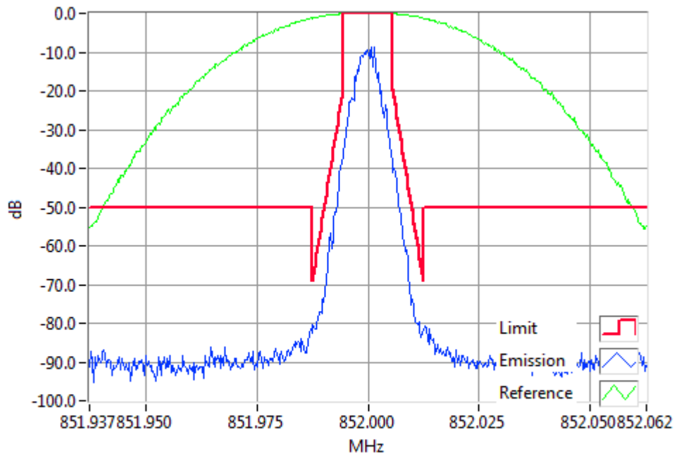
DMR 852.0000MHz Mask D 1W RBW=100Hz, VBW=1000Hz, Detector Mode=Peak Result=Pass
