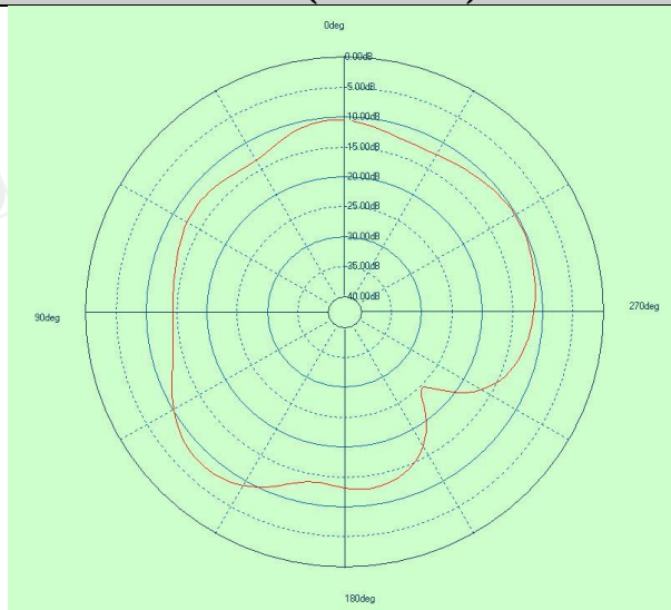
Free Space GAIN TOTAL (5800MHz) – YZ cut
