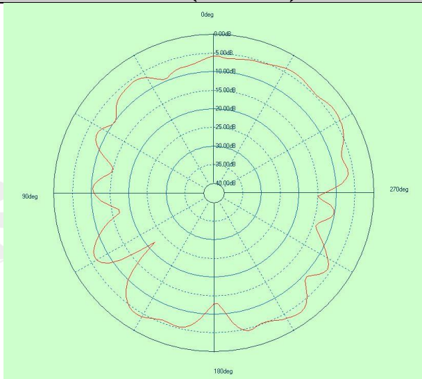
Free Space GAIN TOTAL (5800MHz) – XZ cut
