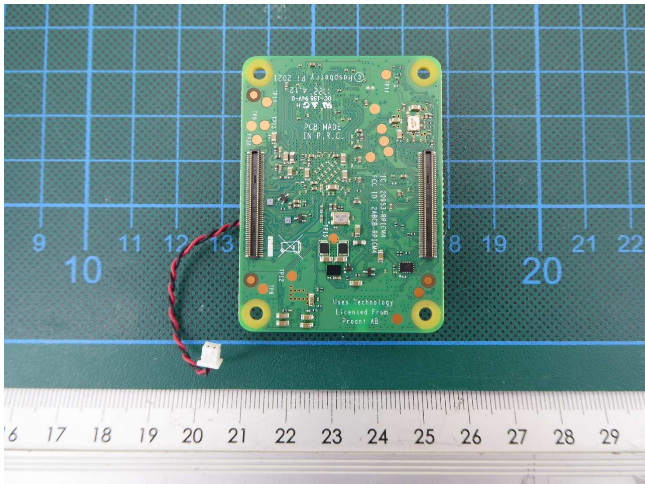
Host Raspberry Pi PCB bottom view
