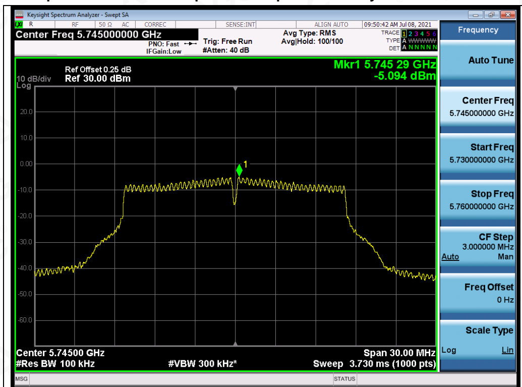
Test_Graph_802.11a_ANT1_5745_6Mbps_PSD
