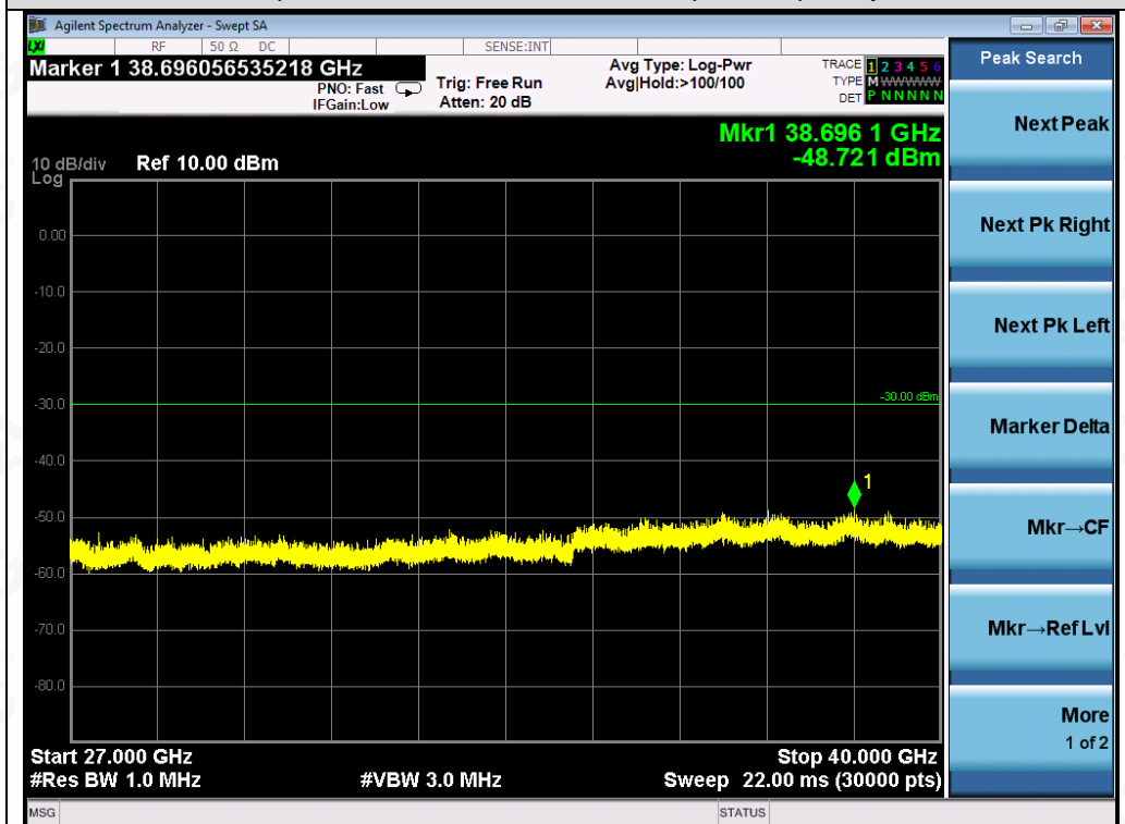
Test_Graph_802.11a_ANT1_5260_6Mbps_Frequency Band 5
