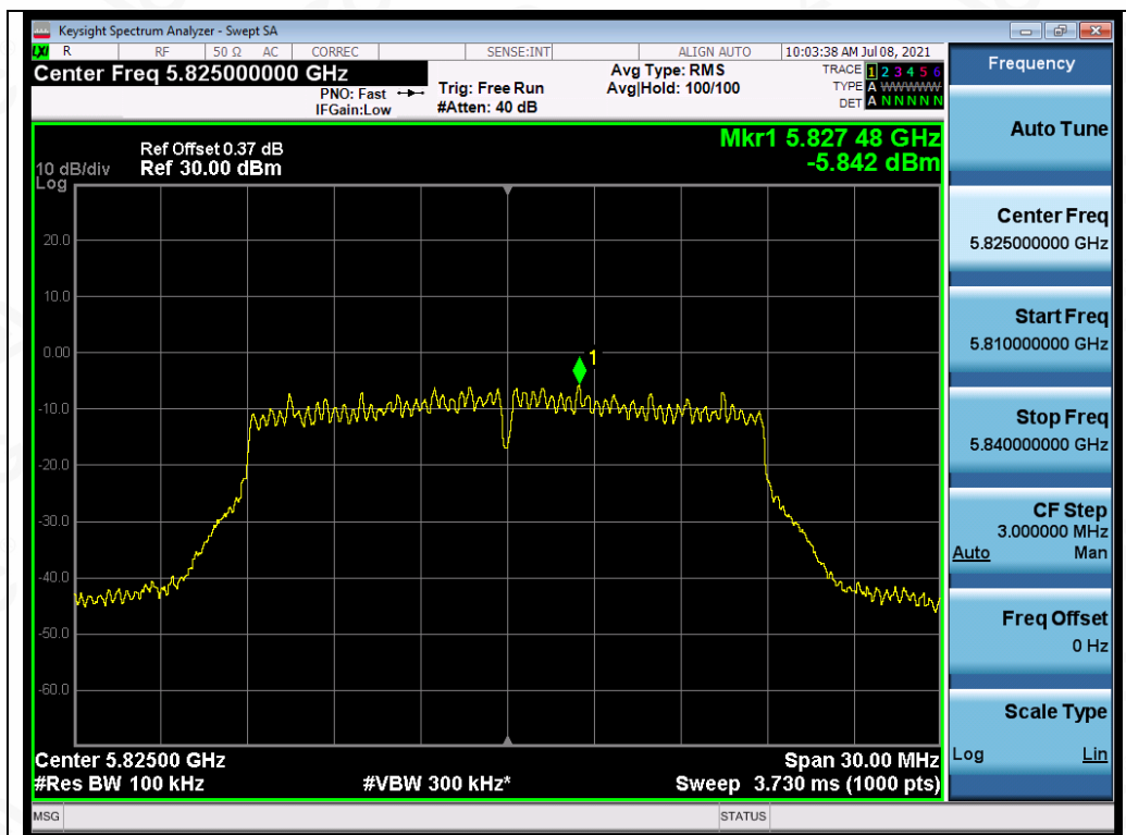
Test_Graph_802.11ac20_ANT1_5825_MCS9_PSD
