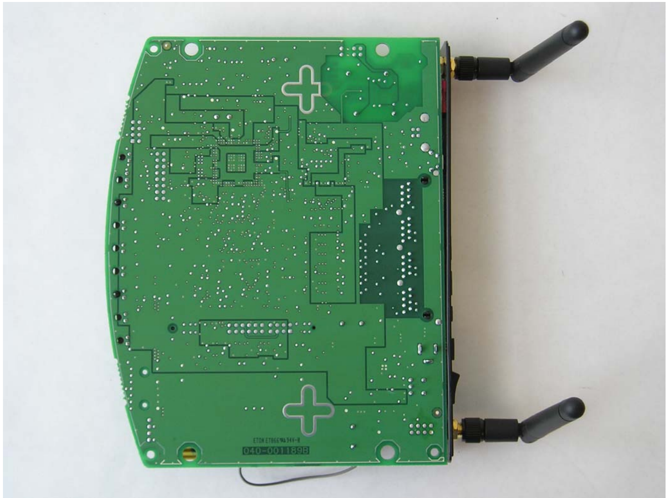
Photo of Main PCB: Foil Side
