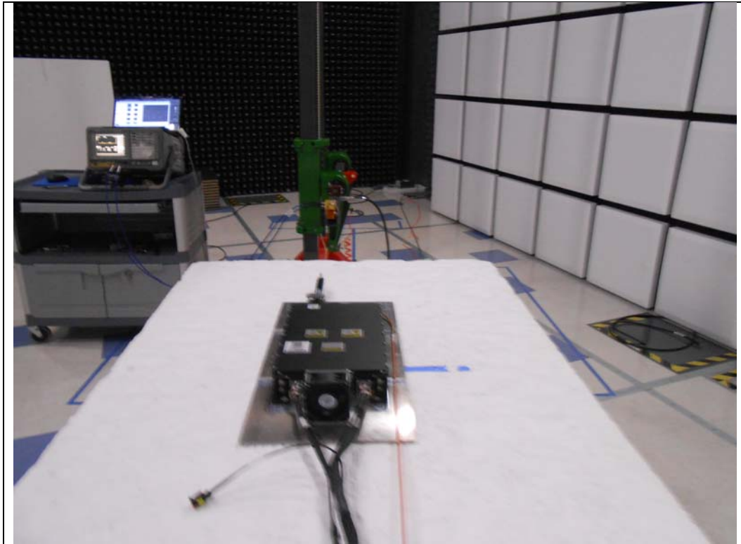
RF Radiated above 1 GHz with 50 ohm Load #2
