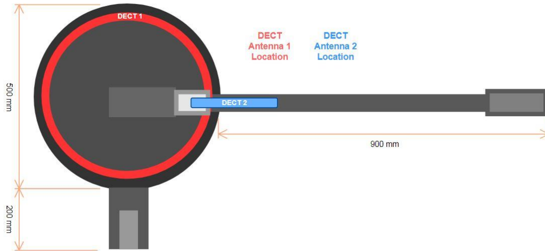
Fig. 1: Sketches and antenna location of the EUT (marked in red).
