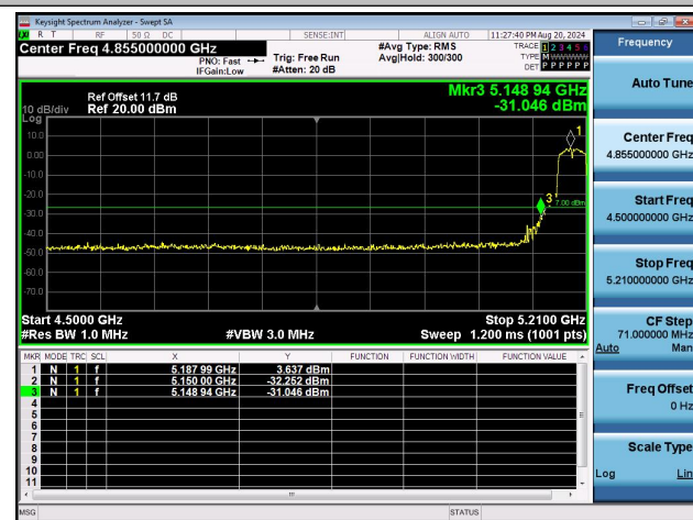
11N40SISO-Ant1-5190-PASS
