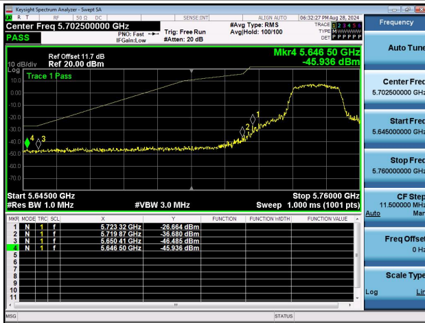
11N20SISO-Ant1-5745-PASS
