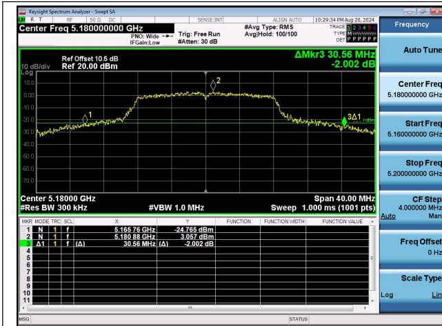
11A-Ant1-5180-26dB EBW
