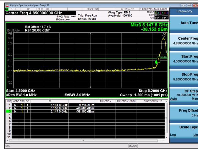
11N20SISO-Ant1-5180-PASS
