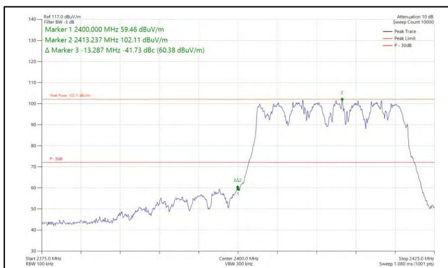
Figure 88 - 802.11ax HE20, SU, CDD, Core 0-1 - 2412 MHz Band Edge Frequency 2400 MHz
