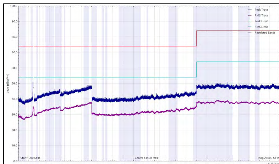
Figure 134 - 2442 MHz (CH7), HE20, RU26-0, CDD, Core 0 + Core 1, 1 GHz to 26 GHz, Horizontal
