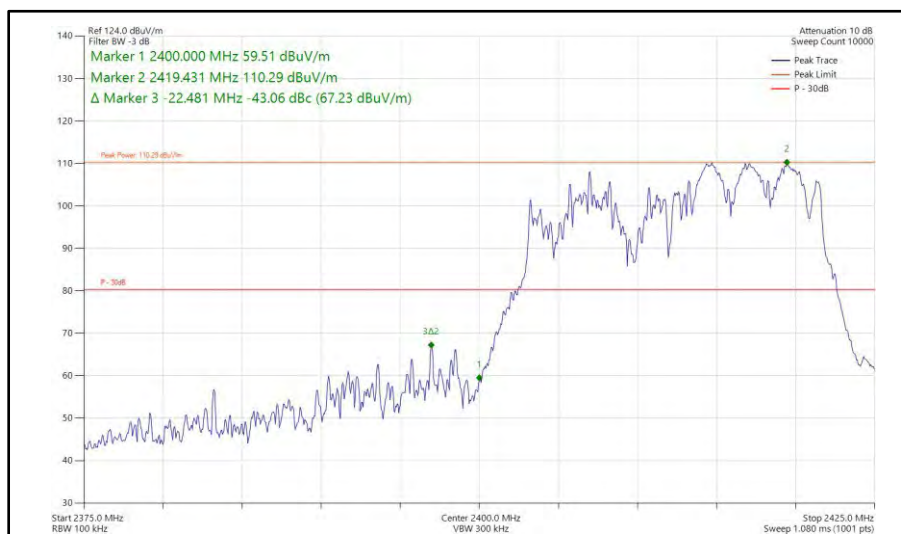
Figure 89 - 802.11ax HE20, RU 106-54, CDD, Core 0-1 - 2412 MHz Band Edge Frequency 2400 MHz
