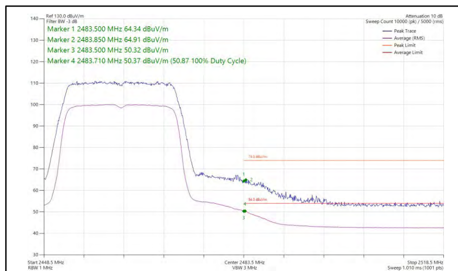
Figure 35 - 802.11ax HE20, SU, SISO, Core 1 - 2462 MHz Band Edge Frequency 2483.5 MHz
