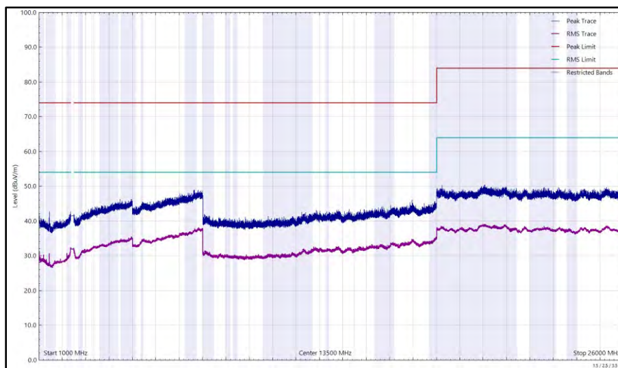
Figure 100 - 2412 MHz (CH1), 802.11b, Core 1, 1 GHz to 26 GHz, Vertical
