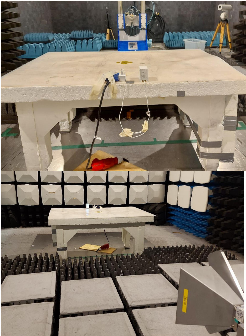
Test set up radiated emission 1 GHz – 12.5 GHz
