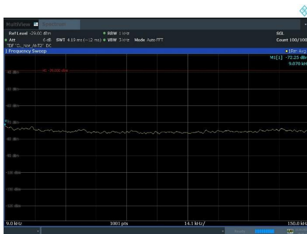
Plot 8-61. Conducted Spurious Emission Plot 9 kHz to 150 kHz (n26_1C_5M_QPSK - Mid Channel, Port 2)
