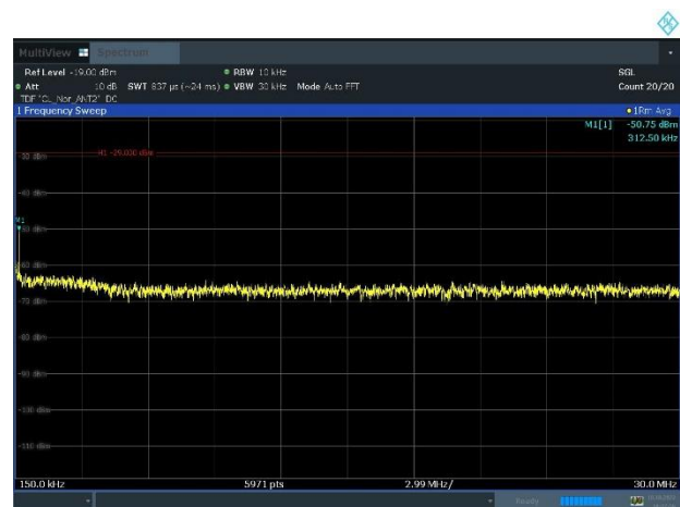
Plot 8-62. Conducted Spurious Emission Plot 150 kHz to 30 MHz (n26_1C_5M_QPSK - Mid Channel, Port 2)
