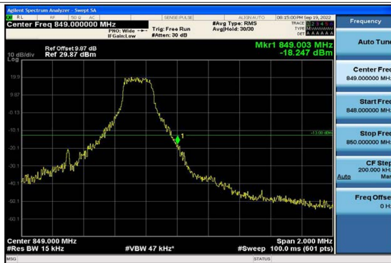
Band5-1.4MHz-QPSK-20643-1RB#5
