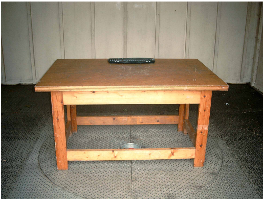
Photograph page 1: Test set up Y-RQ52: on turntable
