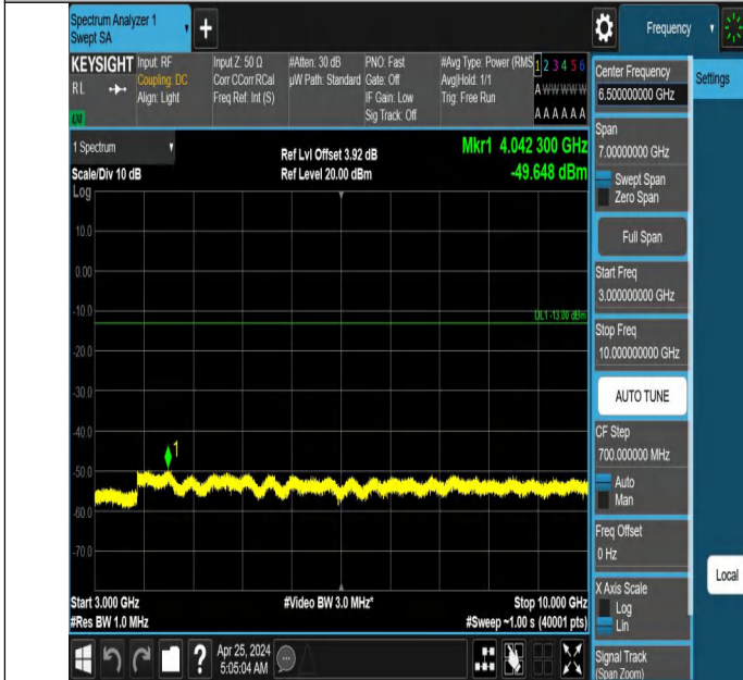
Band71_15MHz_QPSK_133197_1RB#0_3000~10000_3000~1000
