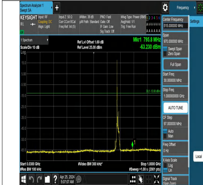
Band71_15MHz_QPSK_133397_1RB#0_30~1000_30~1000
