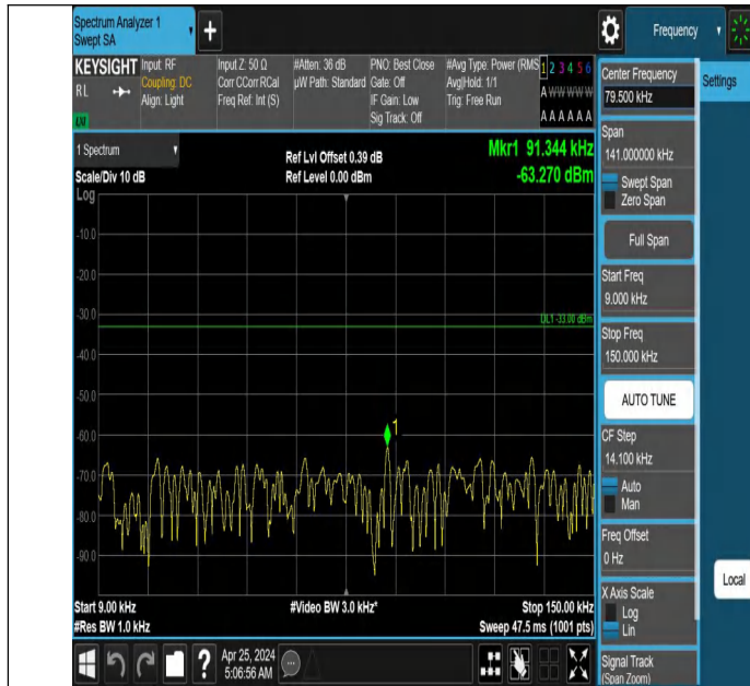
Band71_15MHz_QPSK_133397_1RB#0_0.009~0.15_0.009~0.15
