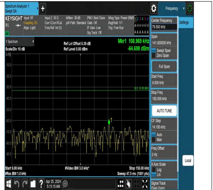
Band71_20MHz_QPSK_133222_1RB#0_0.009~0.15_0.009~0.15
