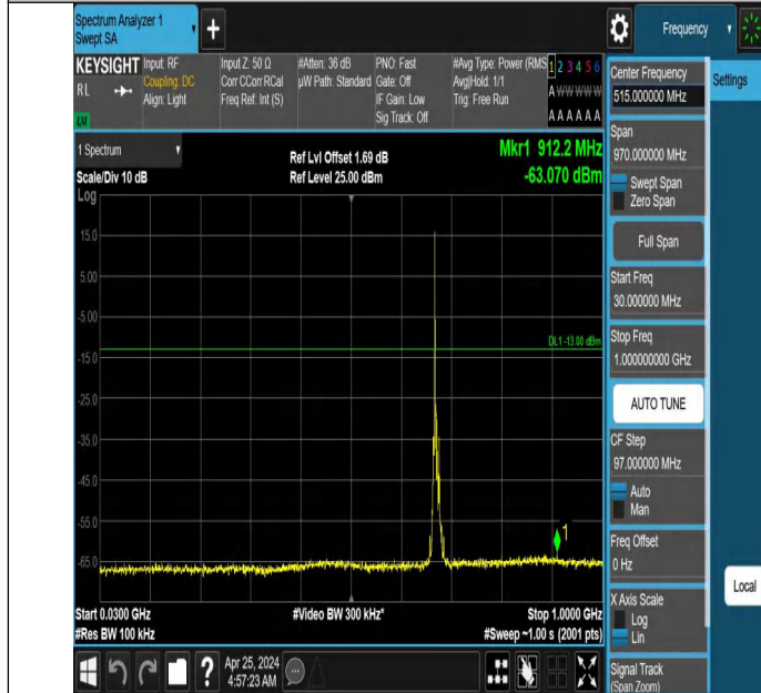
Band71_10MHz_QPSK_133297_1RB#0_30~1000_30~1000
