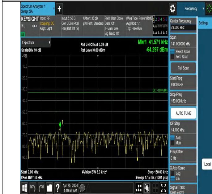
Band71_5MHz_QPSK_133447_1RB#0_0.009~0.15_0.009~0.15
