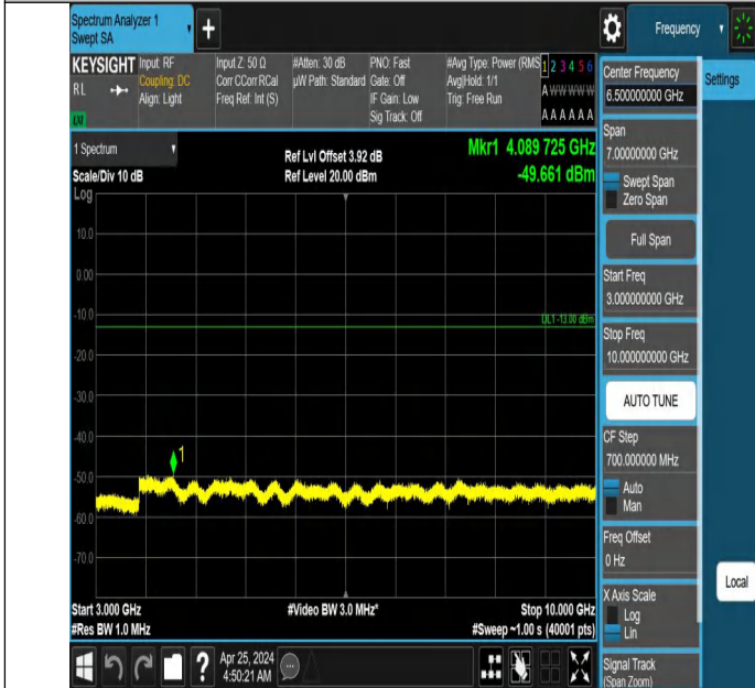
Band71_5MHz_QPSK_133447_1RB#0_3000~10000_3000~1000
