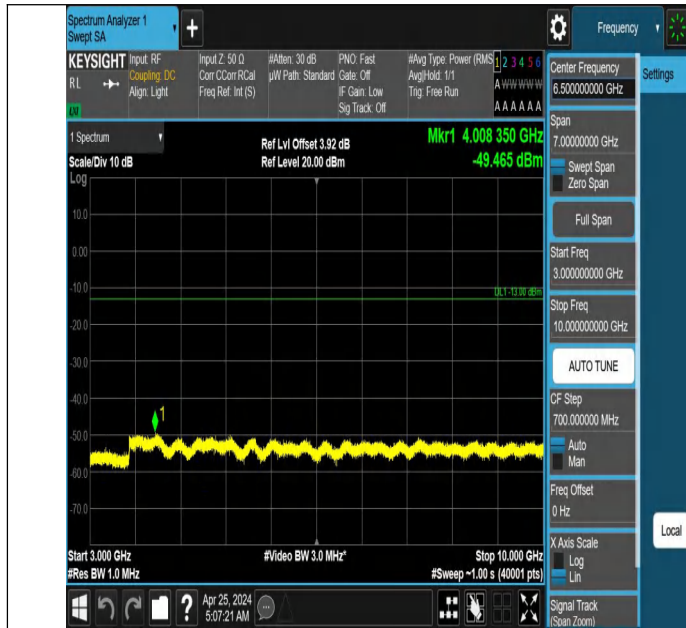
Band71_15MHz_QPSK_133397_1RB#0_3000~10000_3000~10000
