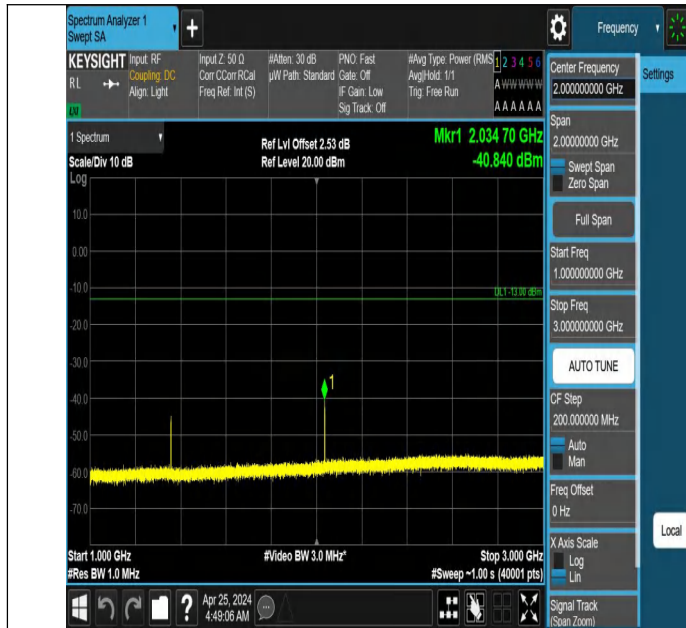
Band71_5MHz_QPSK_133297_1RB#0_1000~3000_1000~3000
