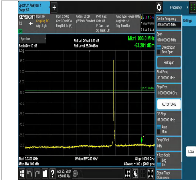
Band71_5MHz_QPSK_133447_1RB#0_30~1000_30~1000
