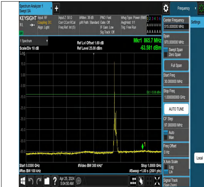
Band71_15MHz_QPSK_133197_1RB#0_30~1000_30~1000
