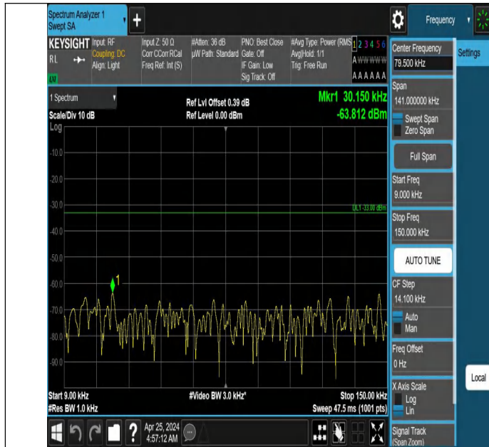
Band71_10MHz_QPSK_133297_1RB#0_0.009~0.15_0.009~0.15
