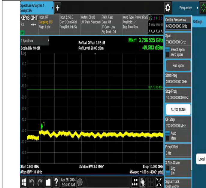
Band71_20MHz_QPSK_133322_1RB#0_3000~10000_3000~1000
