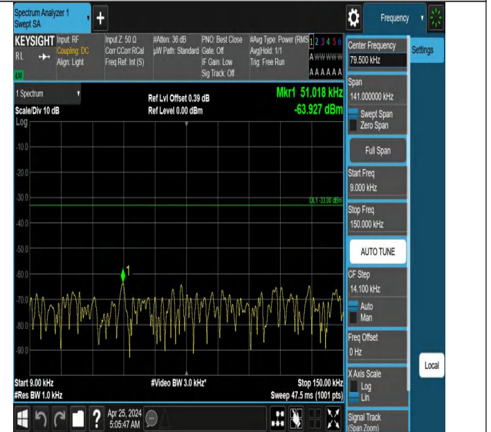
Band71_15MHz_QPSK_133297_1RB#0_0.009~0.15_0.009~0.15
