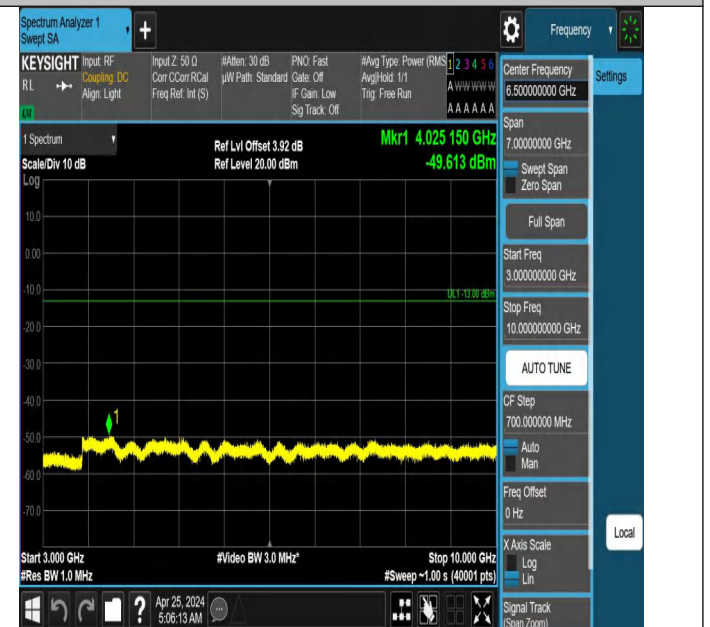
Band71_15MHz_QPSK_133297_1RB#0_3000~10000_3000~10000
