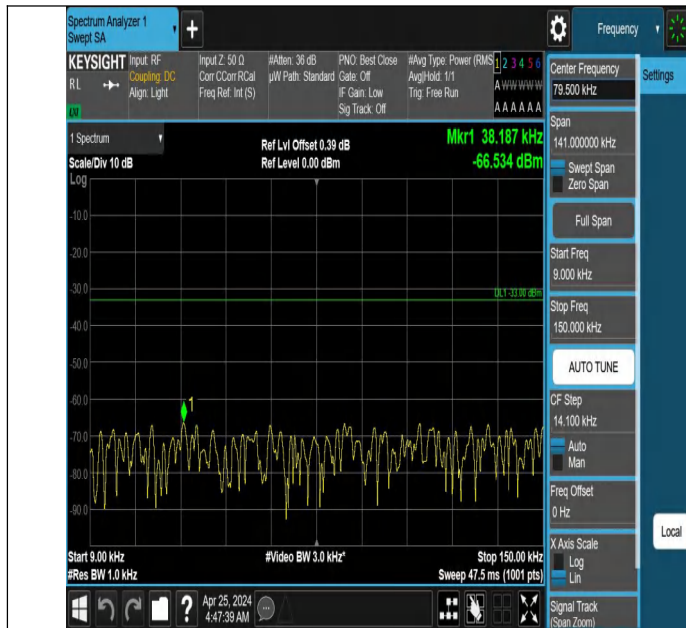
Band71_5MHz_QPSK_133147_1RB#0_0.009~0.15_0.009~0.15
