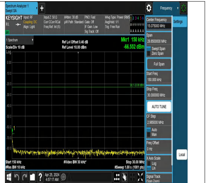
Band71_10MHz_QPSK_133297_1RB#0_0.15~30_0.15~30
