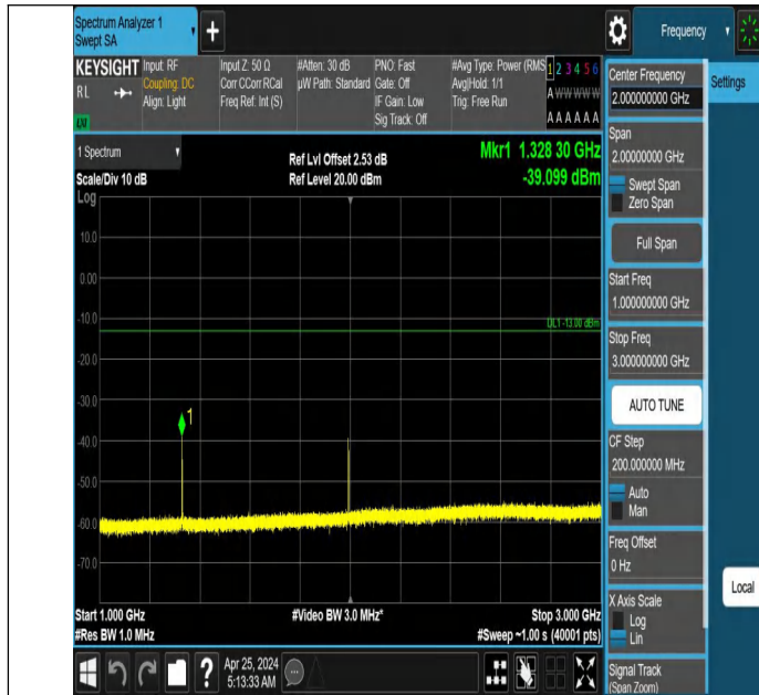
Band71_20MHz_QPSK_133222_1RB#0_1000~3000_1000~3000
