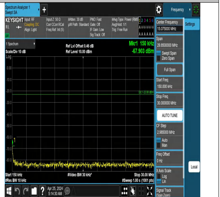
Band71_20MHz_QPSK_133222_1RB#0_0.15~30_0.15~30
