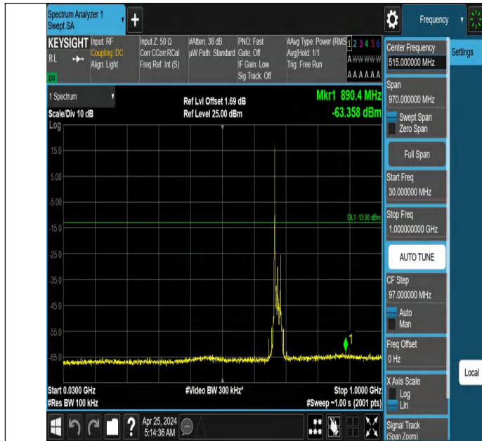
Band71_20MHz_QPSK_133322_1RB#0_30~1000_30~1000
