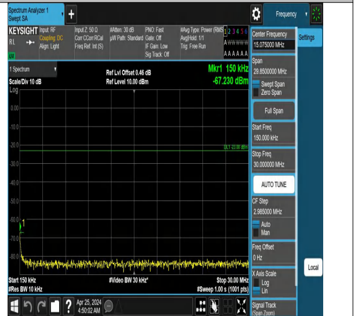
Band71_5MHz_QPSK_133447_1RB#0_0.15~30_0.15~30
