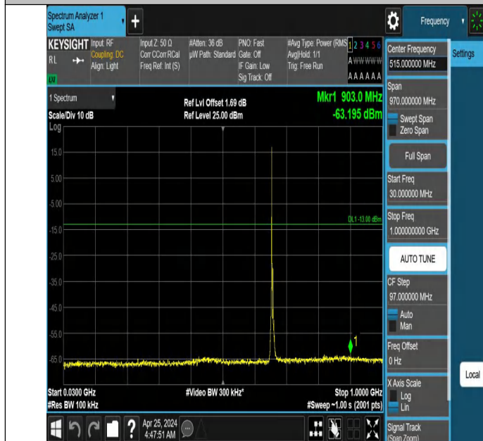
Band71_5MHz_QPSK_133147_1RB#0_30~1000_30~1000
