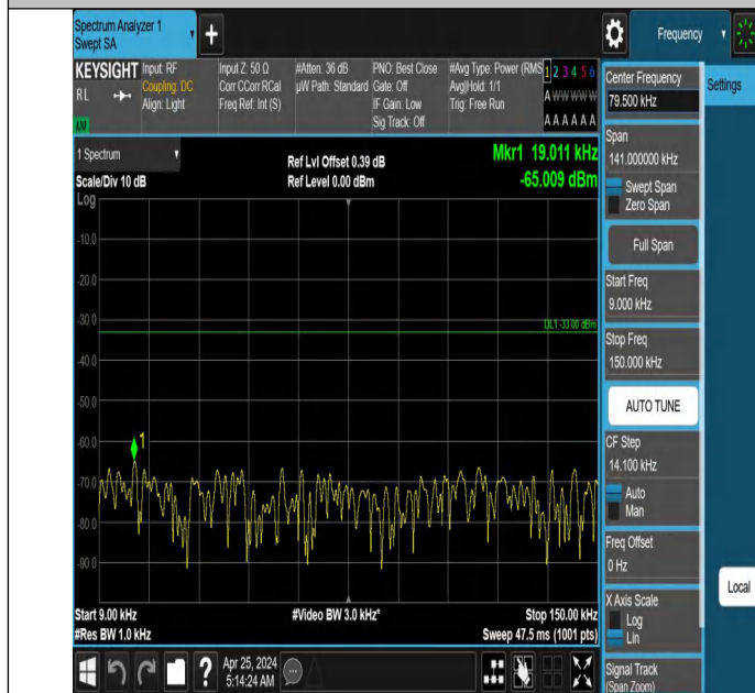
Band71_20MHz_QPSK_133222_1RB#0_0.009~0.15_0.009~0.15
