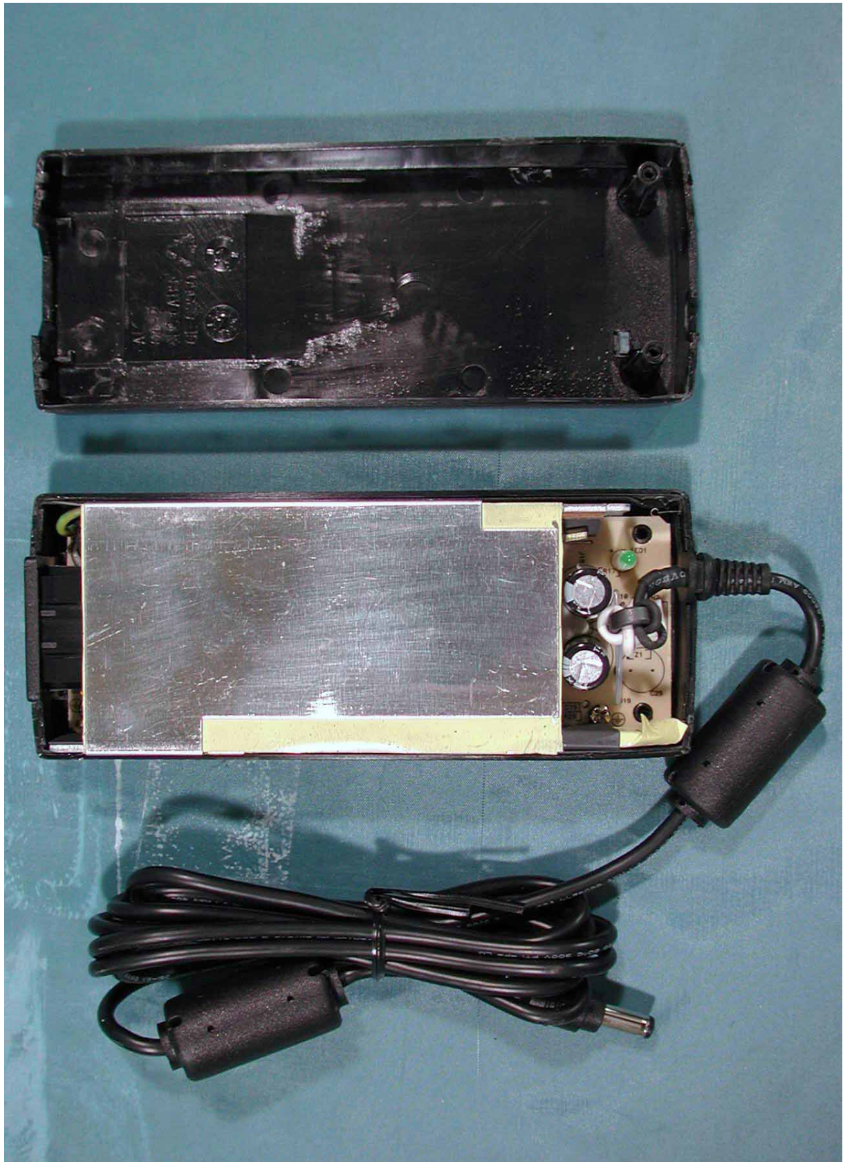
Adapter Assembly
