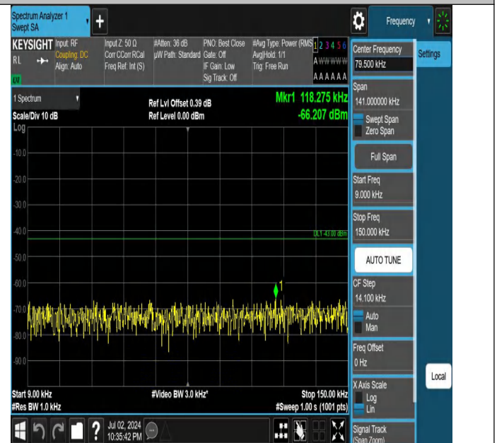
Band4-20MHz-QPSK-20300-1RB#99-0.009~0.15-PASS
