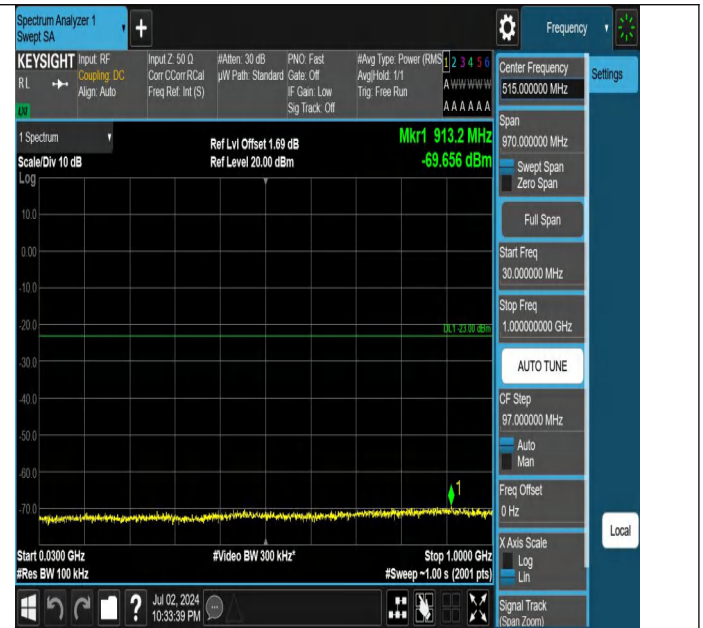
Band4-20MHz-QPSK-20050-1RB#99-30~1000-PASS
