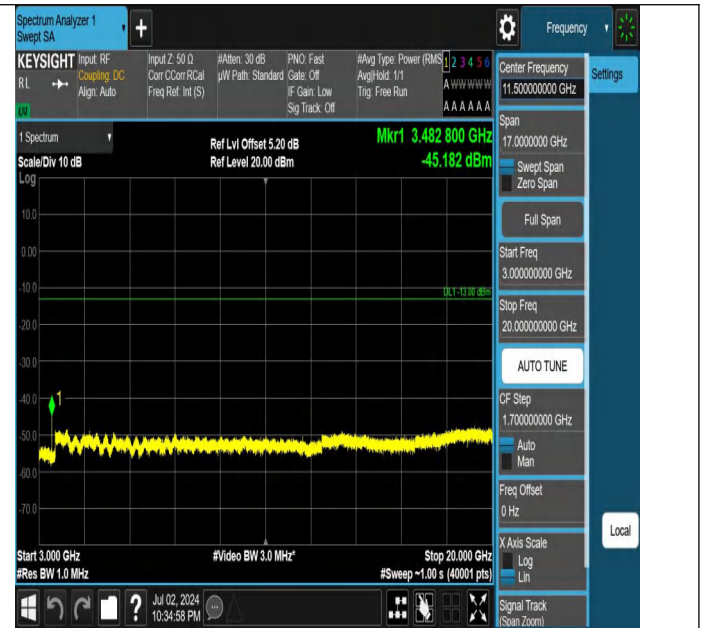
Band4-20MHz-QPSK-20175-1RB#99-3000~20000-PASS
