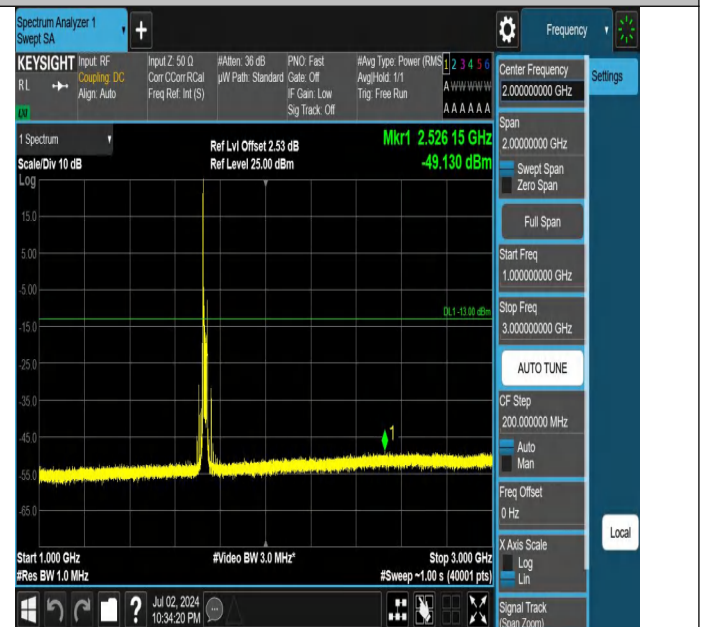
Band4-20MHz-QPSK-20175-1RB#0-1000~3000-PASS
