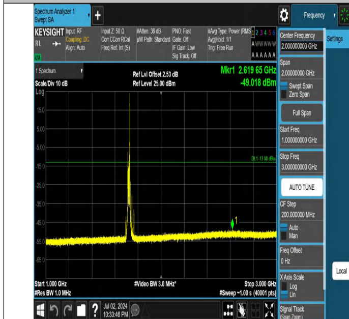
Band4-20MHz-QPSK-20050-1RB#99-1000~3000-PASS
