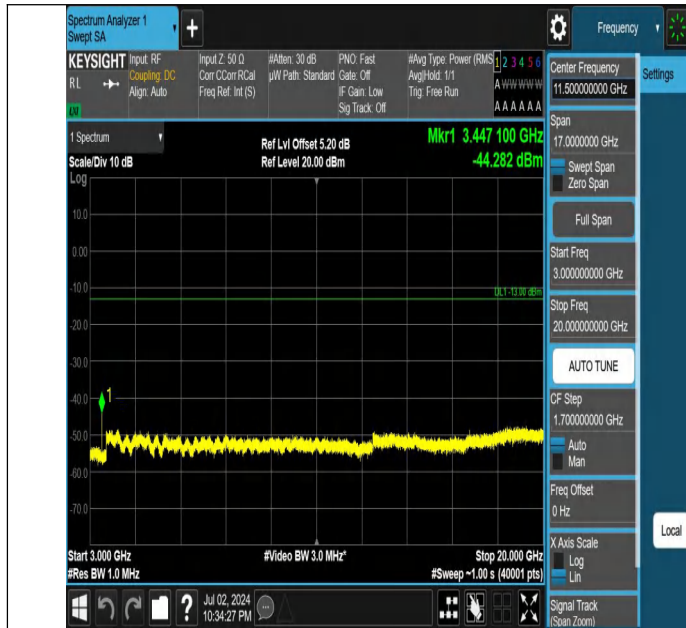
Band4-20MHz-QPSK-20175-1RB#0-3000~20000-PASS
