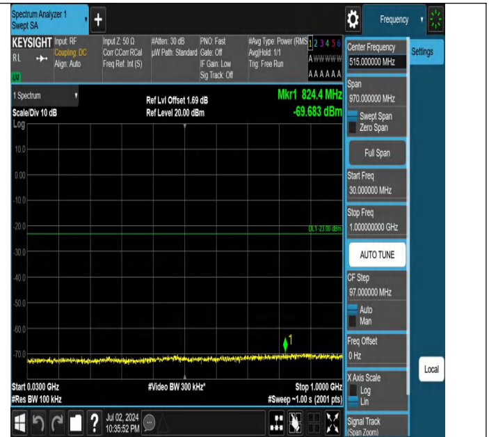
Band4-20MHz-QPSK-20300-1RB#99-30~1000-PASS
