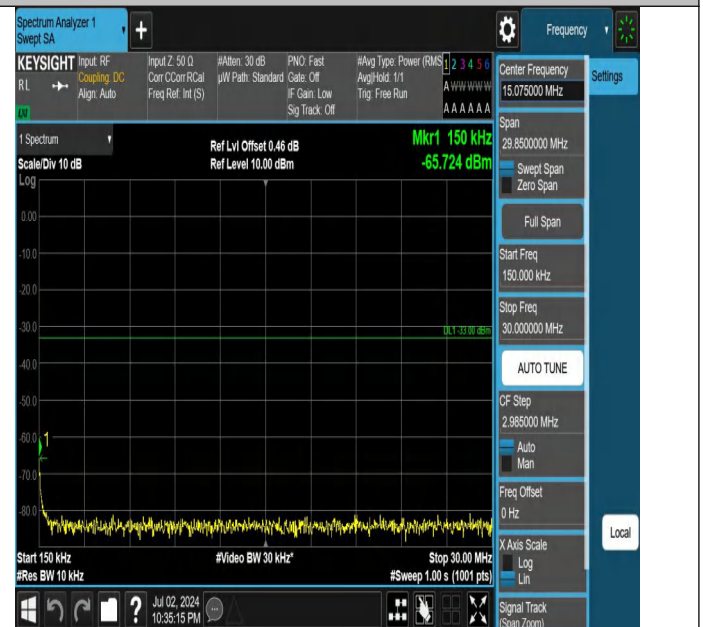
Band4-20MHz-QPSK-20300-1RB#0-0.15~30-PASS
