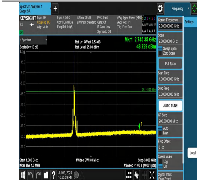
Band4-20MHz-QPSK-20300-1RB#99-1000~3000-PASS
