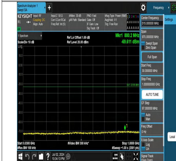
Band4-20MHz-QPSK-20175-1RB#0-30~1000-PASS
