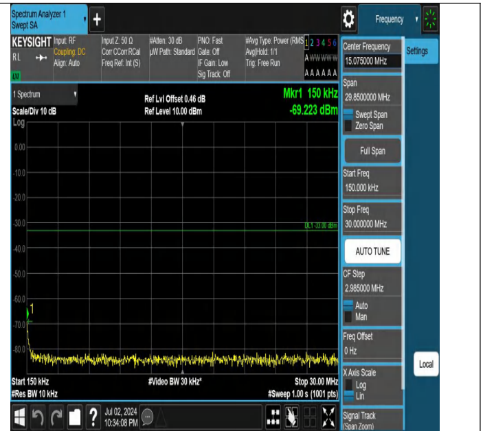
Band4-20MHz-QPSK-20175-1RB#0-0.15~30-PASS
