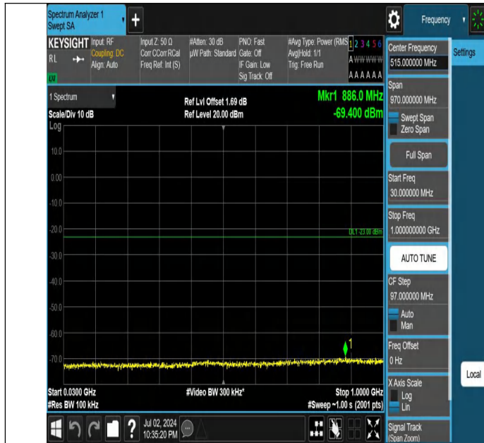
Band4-20MHz-QPSK-20300-1RB#0-30~1000-PASS
