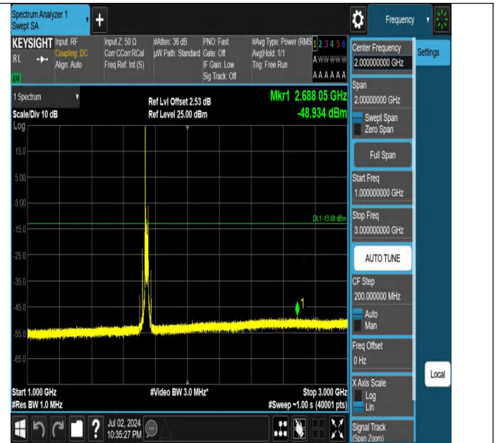
Band4-20MHz-QPSK-20300-1RB#0-1000~3000-PASS
