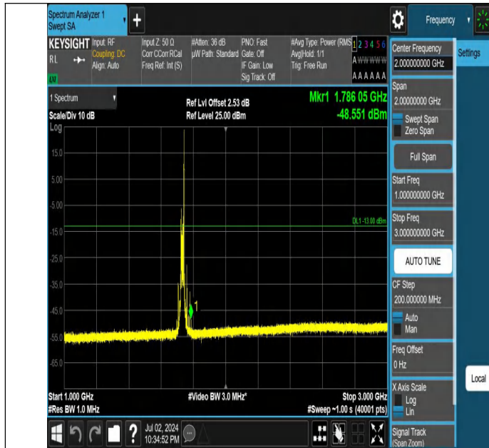
Band4-20MHz-QPSK-20175-1RB#99-1000~3000-PASS
