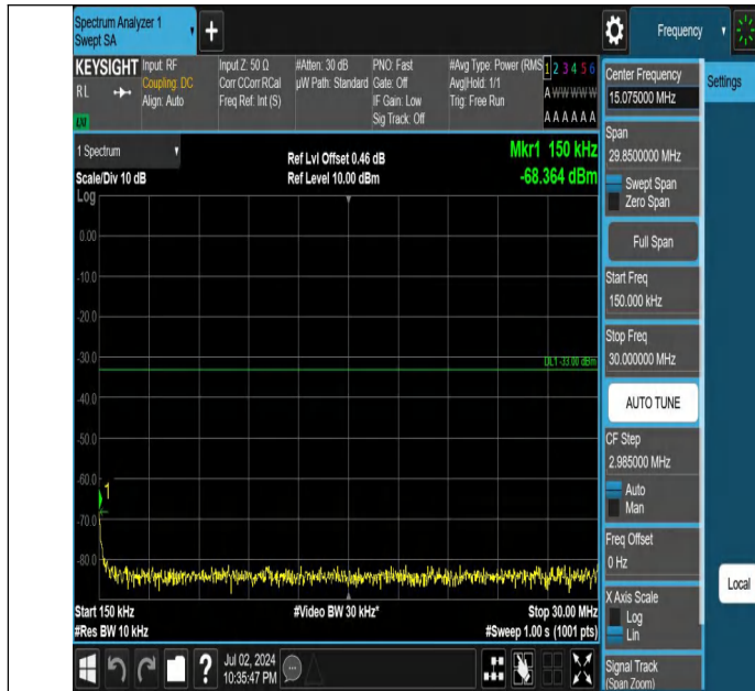
Band4-20MHz-QPSK-20300-1RB#99-0.15~30-PASS
