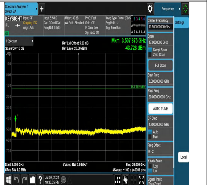
Band4-20MHz-QPSK-20300-1RB#99-3000~20000-PASS
