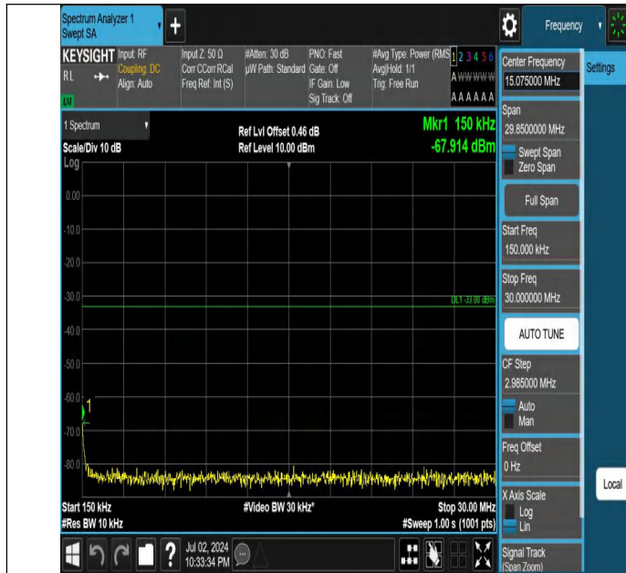
Band4-20MHz-QPSK-20050-1RB#99-0.15~30-PASS
