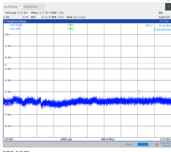
1-N38--30-40-H-1-DFT-PI2BPSK-Inner_1RB_Left-1 @1-3000-12000-Ant0--52.16--25-PASS
