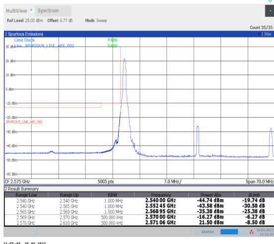
1-N38--30-40-L-4-CP-QPSK-Edge_1RB_Left-1@0-Ant0-PASS-see graph
