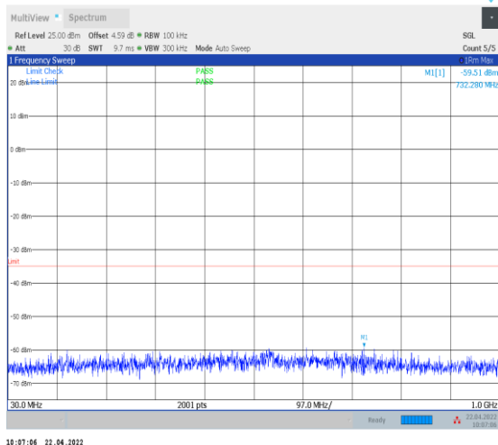
1-N38--30-40-M-1-DFT-PI2BPSK-Inner_1RB_Left-1 @1-30-1000-Ant0--59.51--35-PASS
