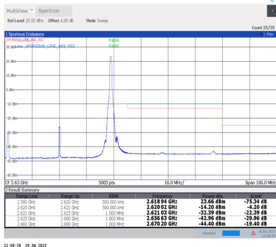
1-N38--30-40-H-2-DFT-PI2BPSK-Edge_1RB_Right-1@105-Ant0-PASS-see graph
