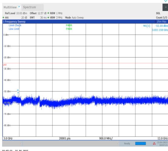
1-N38--30-40-M-1-DFT-PI2BPSK-Inner_1RB_Left-1 @1-3000-12000-Ant0--52.18--25-PASS
