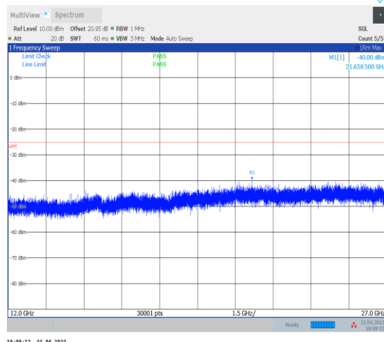
1-N38--30-40-H-1-DFT-PI2BPSK-Inner_1RB_Left-1 @1-12000-27000-Ant0--40.00--25-PASS
