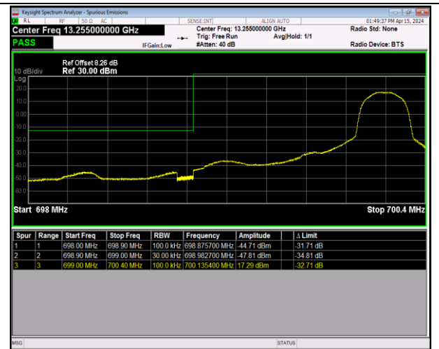
Band12_1.4MHz_64QAM_23017_1RB#5
