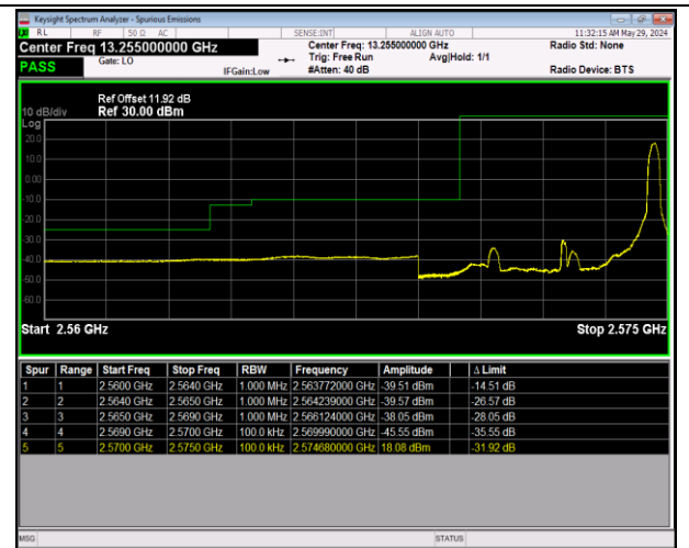
Band38_5MHz_16QAM_37775_1RB#24
