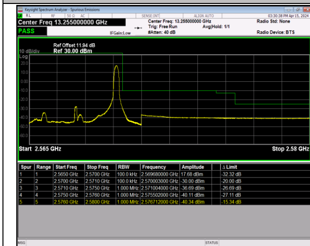
Band7_5MHz_64QAM_21425_1RB#24
