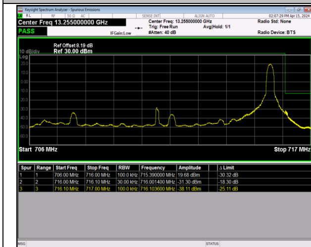
Band12_10MHz_QPSK_23130_1RB#49
