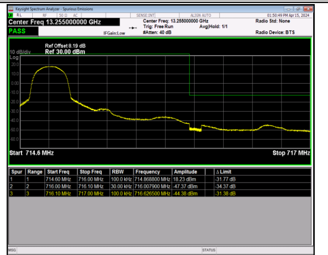
Band12_1.4MHz_16QAM_23173_1RB#5
