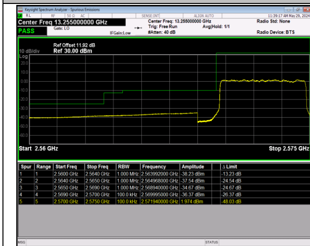
Band38_5MHz_16QAM_37775_25RB#0
