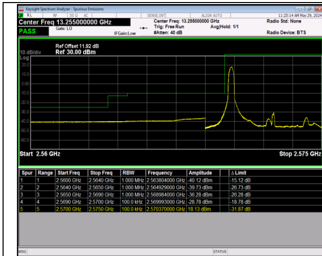
Band38_5MHz_16QAM_37775_1RB#0
