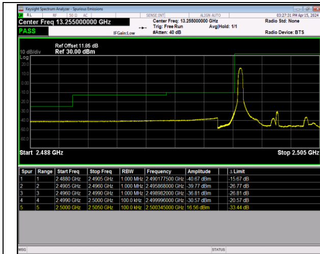
Band7_5MHz_64QAM_20775_1RB#0
