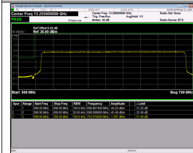
Band12_10MHz_64QAM_23060_50RB#0
