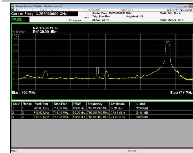
Band12_10MHz_64QAM_23130_1RB#49
