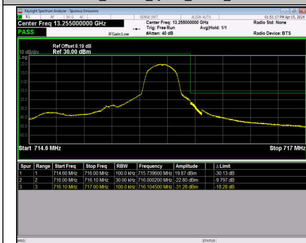
Band12_1.4MHz_QPSK_23173_1RB#5
