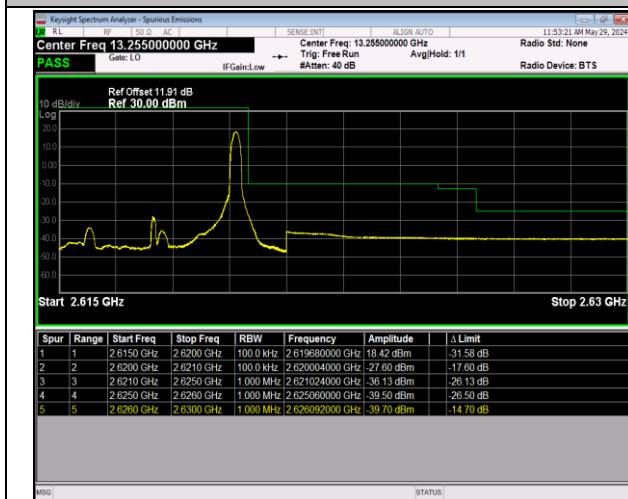
Band38_5MHz_16QAM_38225_1RB#24
