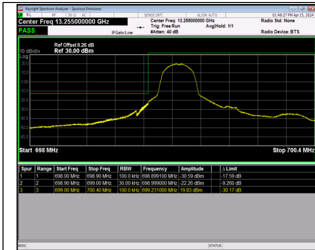
Band12_1.4MHz_QPSK_23017_1RB#0
