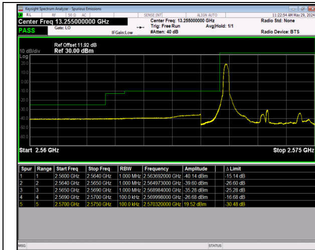
Band38_5MHz_QPSK_37775_1RB#0
