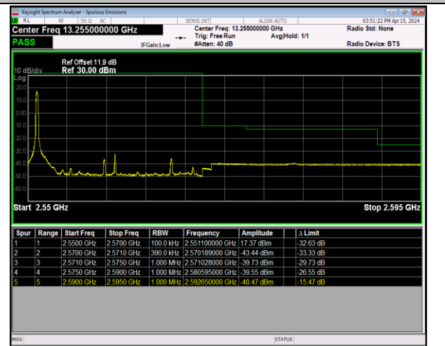
Band7_20MHz_64QAM_21350_1RB#0
