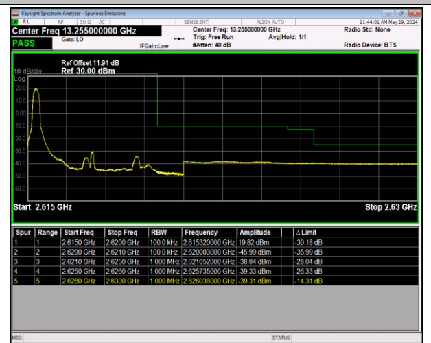
Band38_5MHz_QPSK_38225_1RB#0
