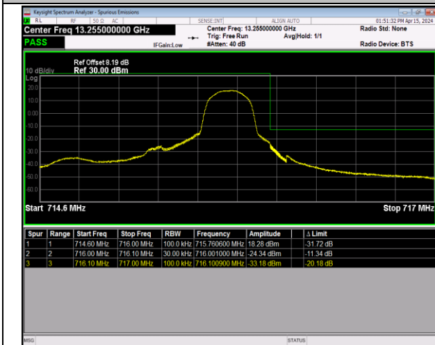
Band12_1.4MHz_16QAM_23173_1RB#0
