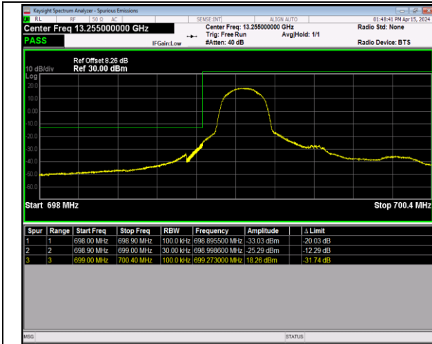
Band12_1.4MHz_16QAM_23017_1RB#0
