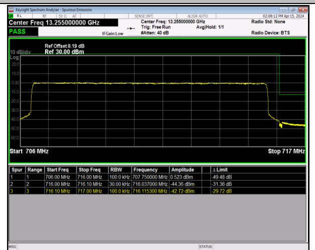
Band12_10MHz_QPSK_23130_50RB#0
