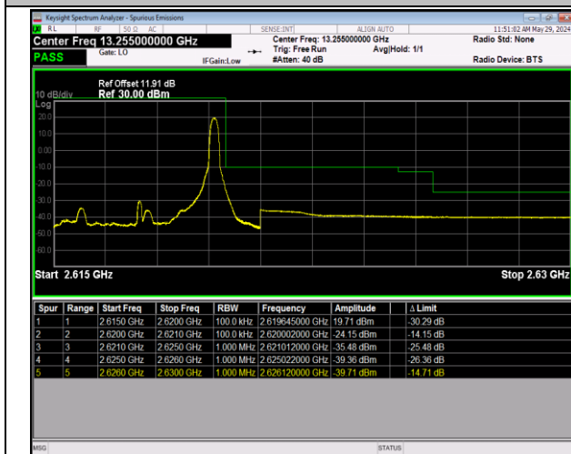
Band38_5MHz_QPSK_38225_1RB#24
