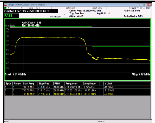
Band12_1.4MHz_64QAM_23173_6RB#0
