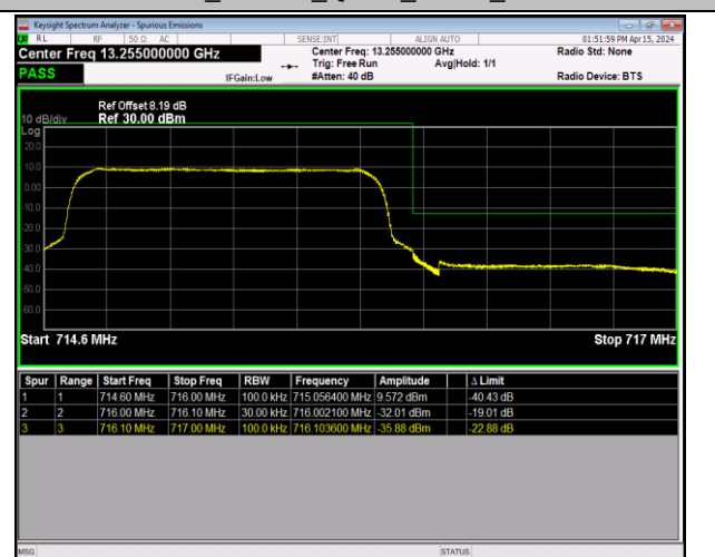
Band12_1.4MHz_QPSK_23173_6RB#0
