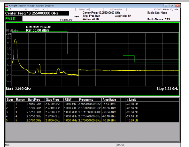
Band7_5MHz_64QAM_21425_1RB#0
