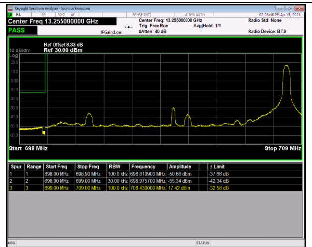
Band12_10MHz_64QAM_23060_1RB#49
