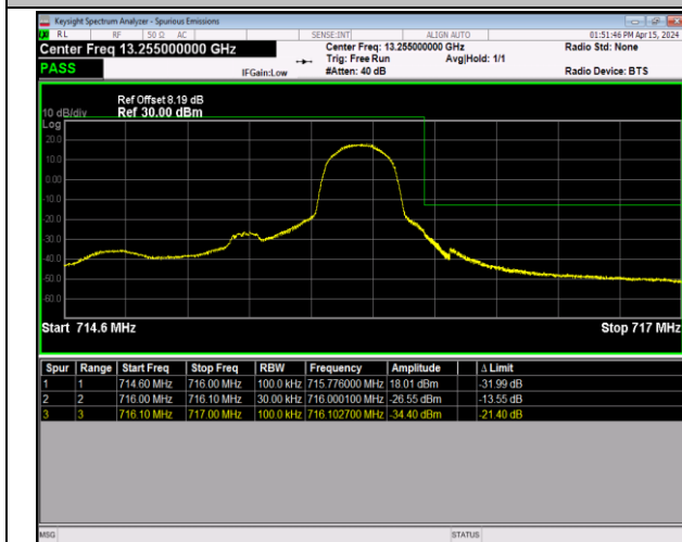
Band12_1.4MHz_64QAM_23173_1RB#5
