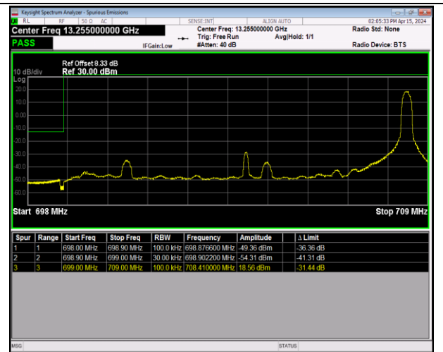
Band12_10MHz_16QAM_23060_1RB#49
