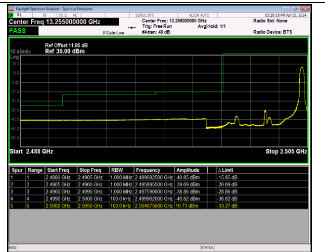
Band7_5MHz_64QAM_20775_1RB#24
