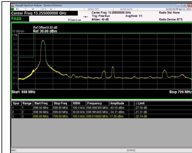
Band12_10MHz_64QAM_23060_1RB#0
