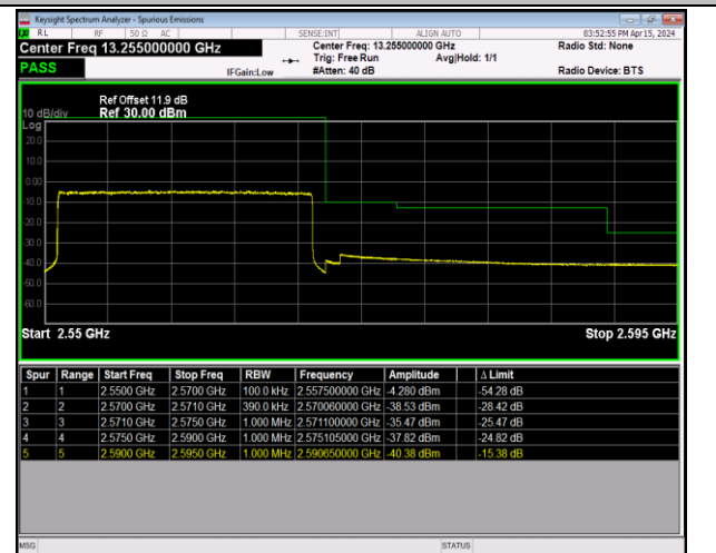
Band7_20MHz_64QAM_21350_100RB#0
