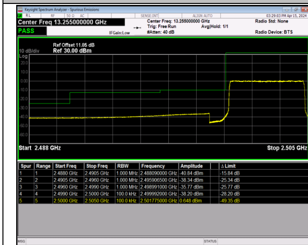
Band7_5MHz_64QAM_20775_25RB#0
