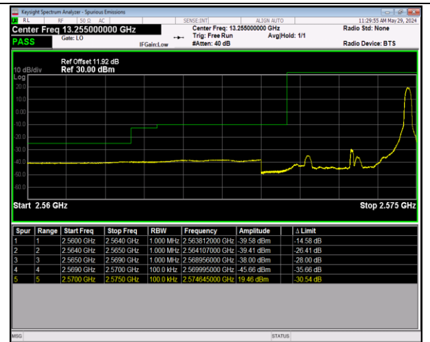
Band38_5MHz_QPSK_37775_1RB#24
