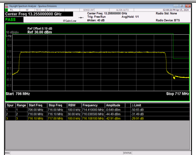
Band12_10MHz_16QAM_23130_50RB#0
