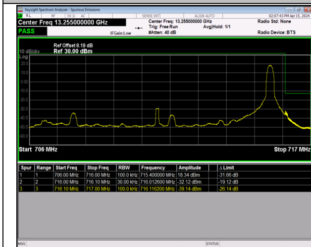
Band12_10MHz_16QAM_23130_1RB#49
