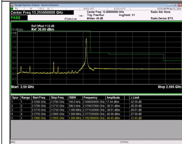
Band7_20MHz_64QAM_21350_1RB#99
