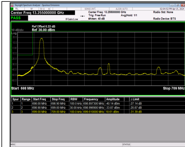
Band12_10MHz_16QAM_23060_1RB#0
