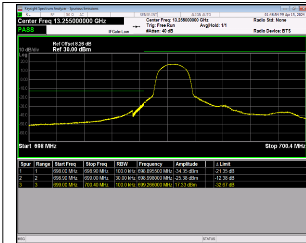
Band12_1.4MHz_64QAM_23017_1RB#0
