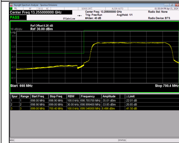
Band12_1.4MHz_16QAM_23017_6RB#0
