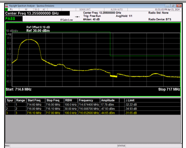
Band12_1.4MHz_64QAM_23173_1RB#0
