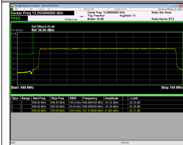
Band12_10MHz_16QAM_23060_50RB#0
