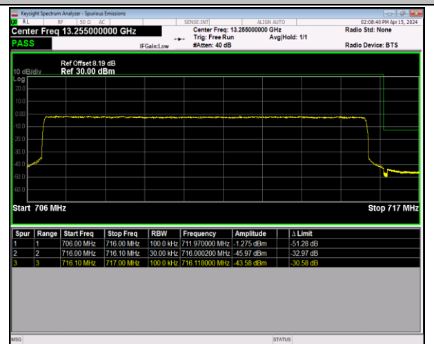
Band12_10MHz_64QAM_23130_50RB#0
