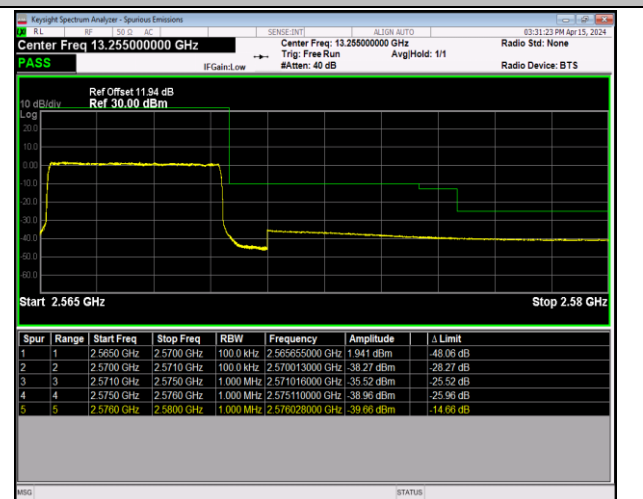
Band7_5MHz_64QAM_21425_25RB#0
