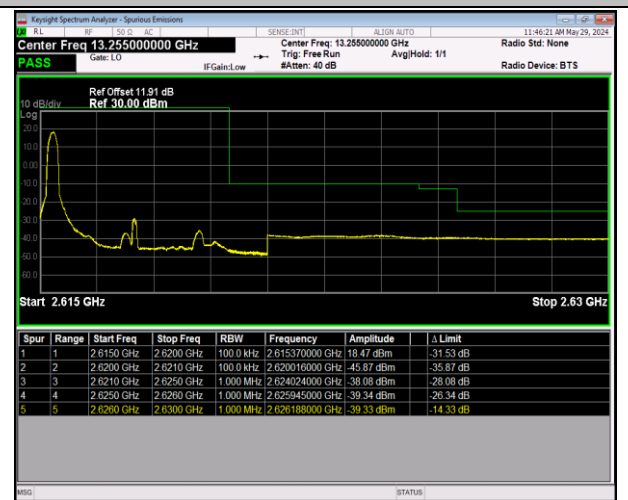
Band38_5MHz_16QAM_38225_1RB#0
