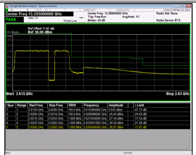
Band38_5MHz_16QAM_38225_25RB#0
