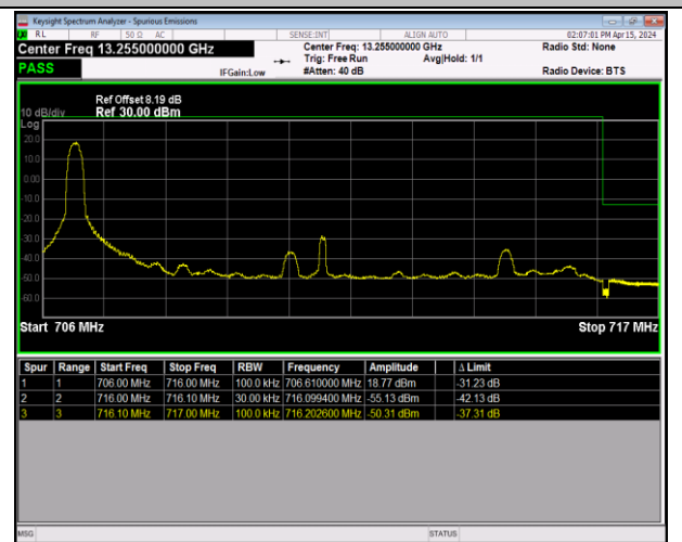
Band12_10MHz_16QAM_23130_1RB#0
