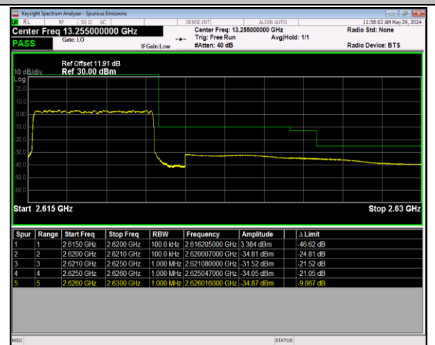
Band38_5MHz_QPSK_38225_25RB#0
