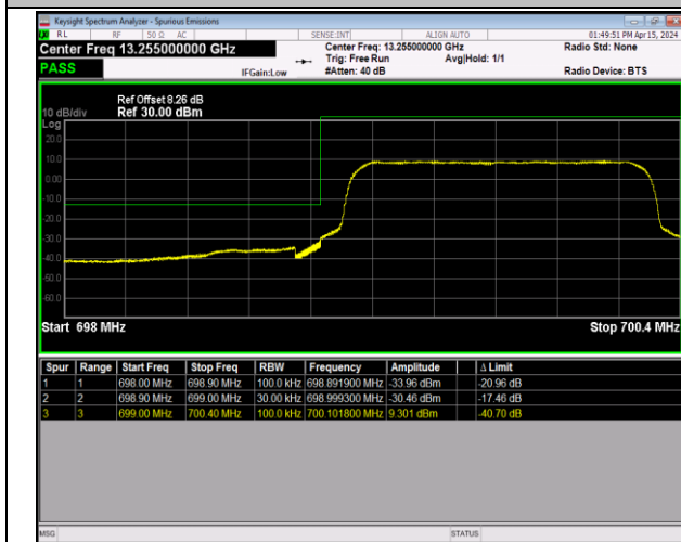
Band12_1.4MHz_QPSK_23017_6RB#0
