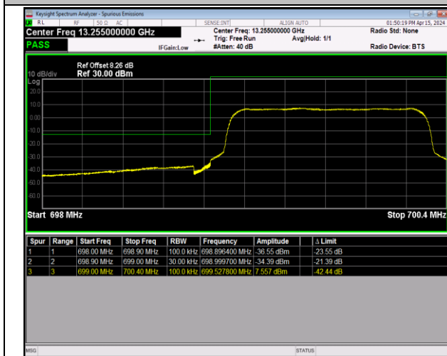
Band12_1.4MHz_64QAM_23017_6RB#0
