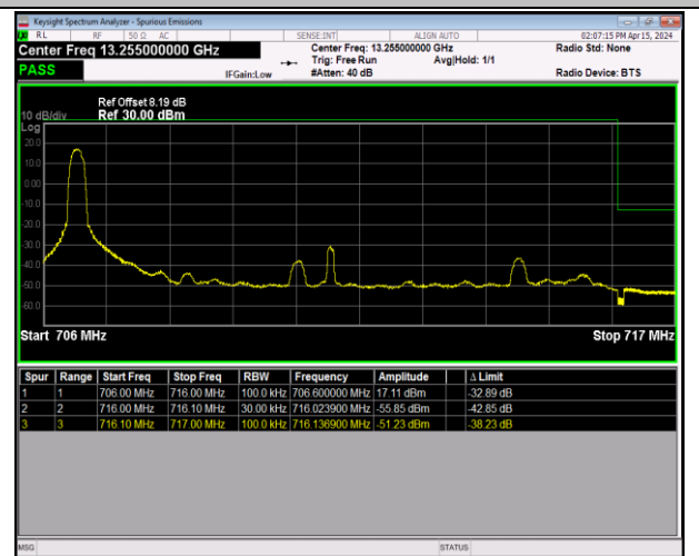
Band12_10MHz_64QAM_23130_1RB#0
