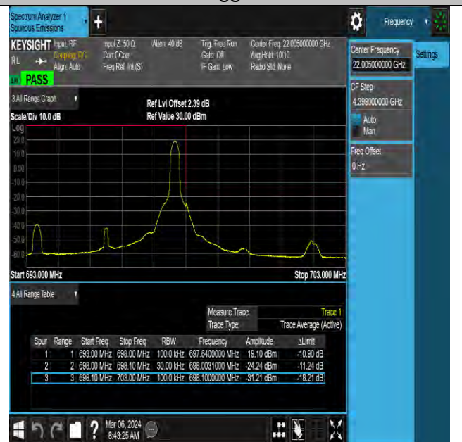
NTNV-N71-PC3-15-5-H-DFT-QPSK-Edge_1RB_Right-Ant0-PASS
