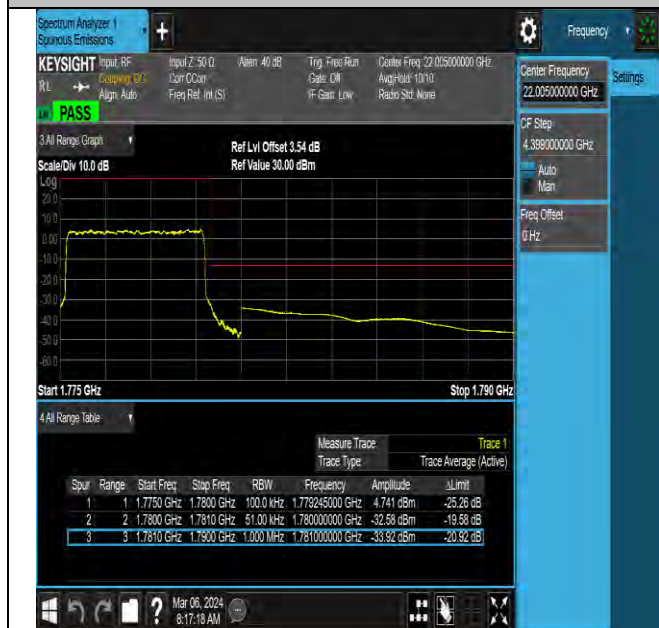
NTNV-N66-PC3-15-5-H-DFT-QPSK-Outer_Full-Ant1-PASS
