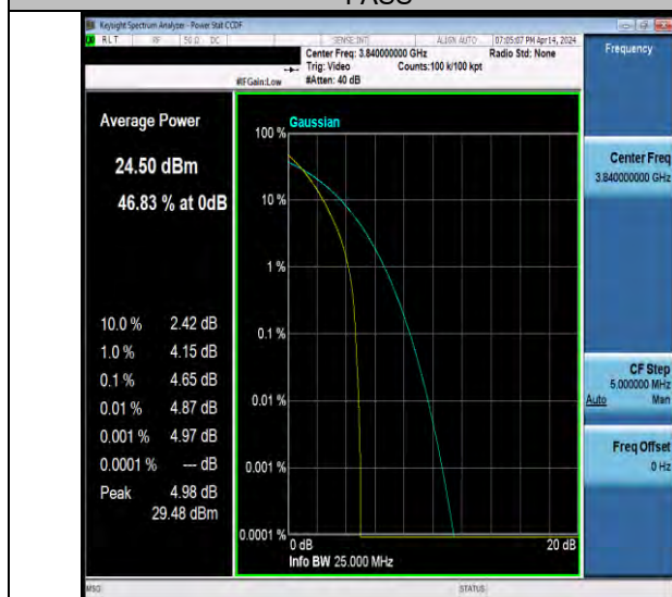
NTNV-N77-3700-3980-PC2-30-20-M-DFT-QPSK-Outer_Full-PASS
