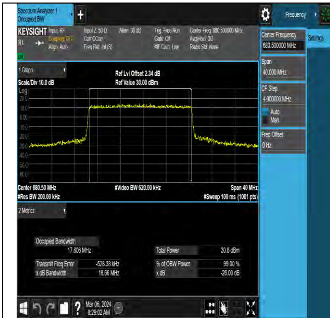
NTNV-N71-PC3-15-20-M-DFT-QPSK-Outer_Full-Ant0-PASS
