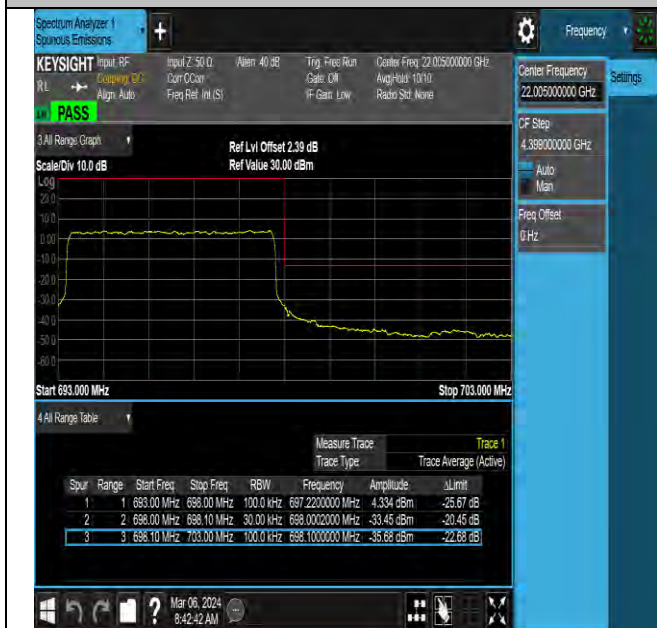
NTNV-N71-PC3-15-5-H-DFT-QPSK-Outer_Full-Ant0-PASS
