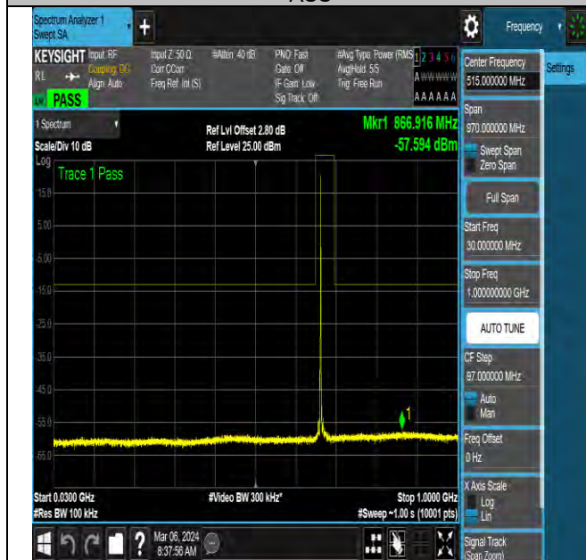
NTNV-N71-PC3-15-20-M-DFT-QPSK-Edge_1RB_Left-Ant0-P PASS
