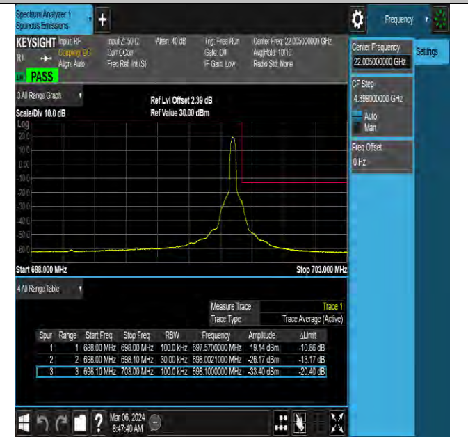
NTNV-N71-PC3-15-10-H-DFT-QPSK-Edge_1RB_Right-Ant0 -PASS
