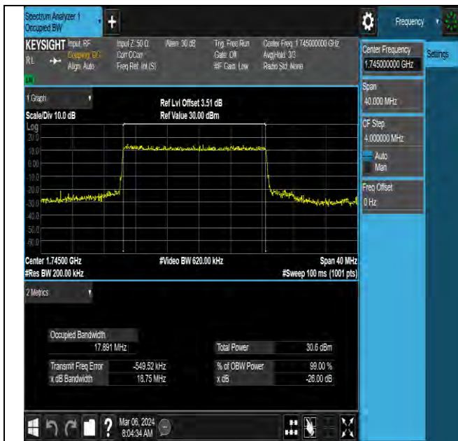
NTNV-N66-PC3-15-20-M-DFT-QPSK-Outter_Full-Ant1-PASS
