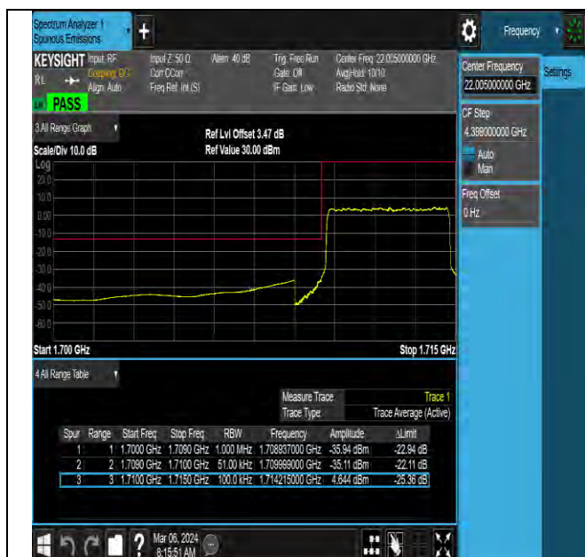
NTNV-N66-PC3-15-5-L-DFT-QPSK-Outer_Full-Ant1-PASS
