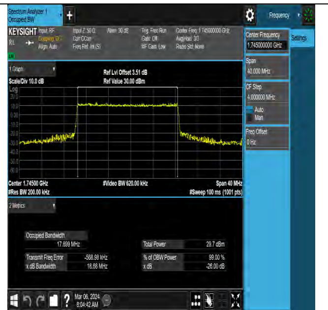
NTNV-N66-PC3-15-20-M-DFT-16QAM-Outter_Full-Ant1-PAS S
