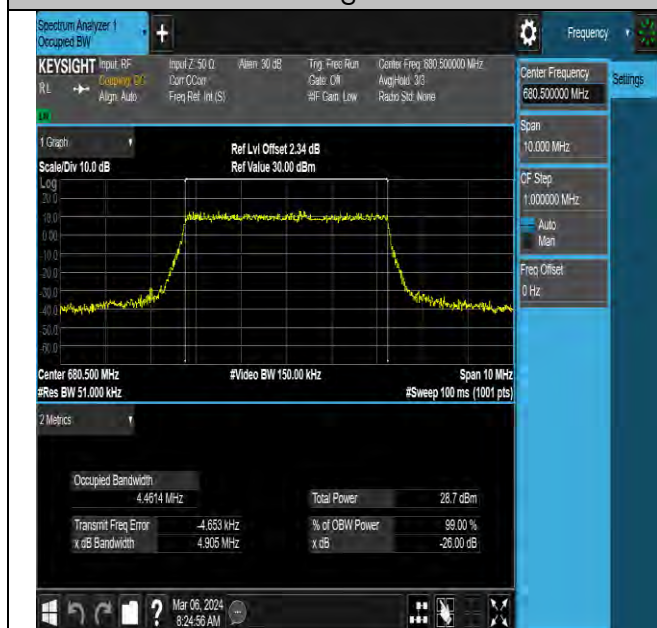
NTNV-N71-PC3-15-5-M-DFT-16QAM-Outet_Full-Ant0-PASS
