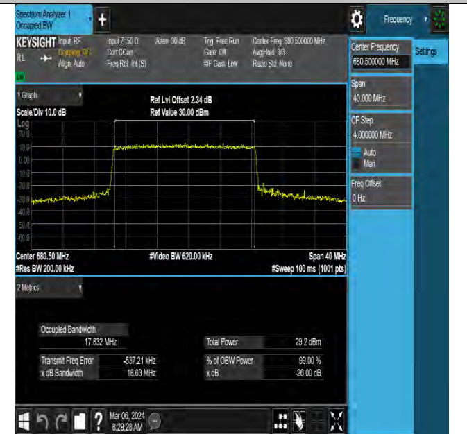
NTNV-N71-PC3-15-20-M-DFT-256QAM-Outer_Full-Ant0-PASS
