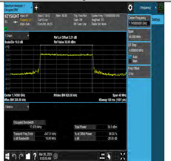
NTNV-N66-PC3-15-20-M-DFT-256QAM-Outter_Full-Ant1-PAS SS
