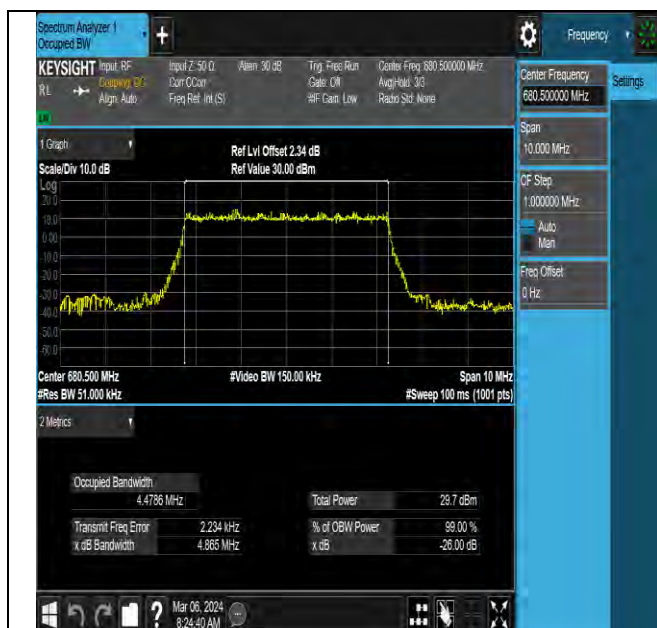
NTNV-N71-PC3-15-5-M-DFT-PI2BPSK-Outet_Full-Ant0-PASS S
