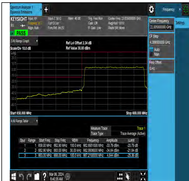
NTNV-N71-PC3-15-5-L-DFT-QPSK-Outer_Full-Ant0-PASS
