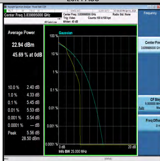
NTNV-N77-3700-3980-PC2-30-20-M-DFT-QPSK-Edge_1RB_Left-PASS
