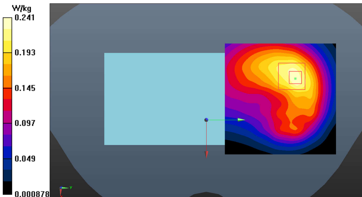
Fig.6 GSM 1900
