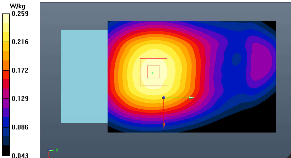
Fig.24 LTE Band 5
