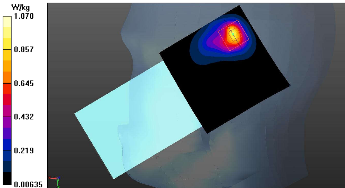
Fig.34 LTE Band 38
