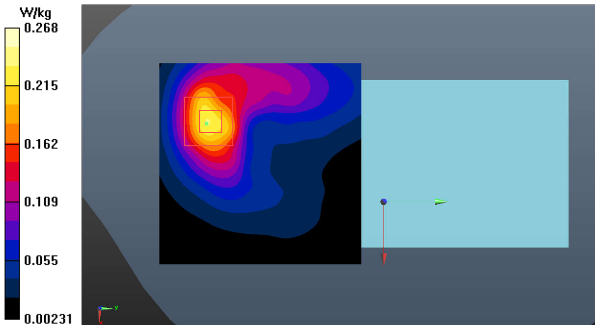
Fig.36 LTE Band 38
