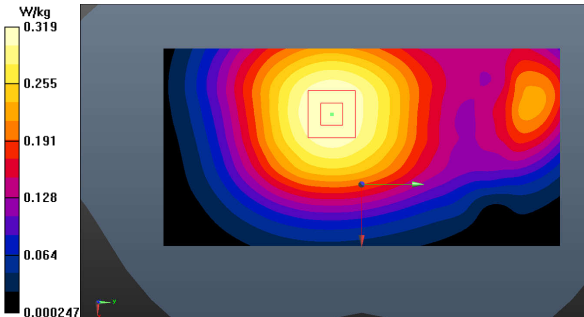
Fig.3 GSM 850
