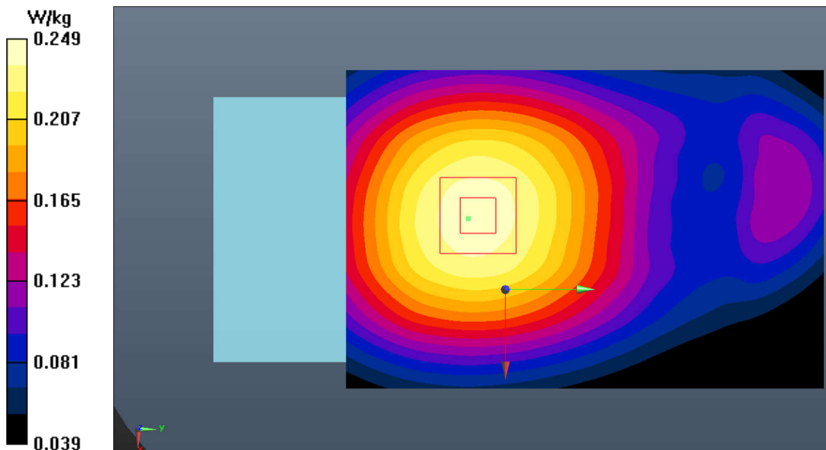
Fig.33 LTE Band 26
