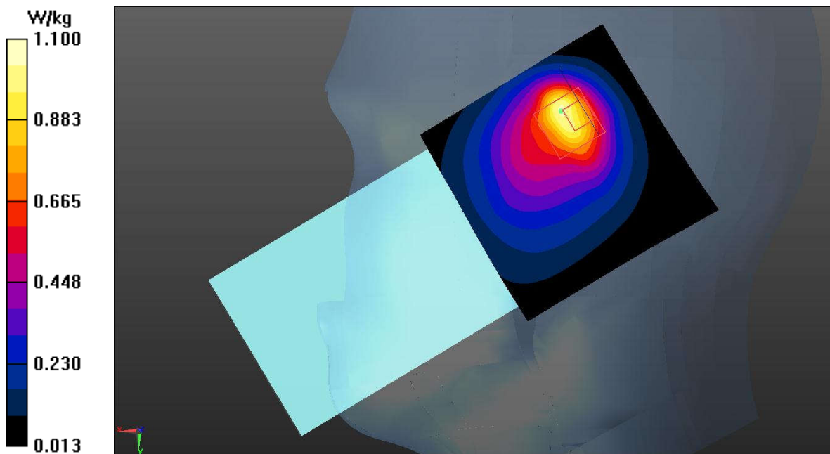
Fig.28 LTE Band 12
