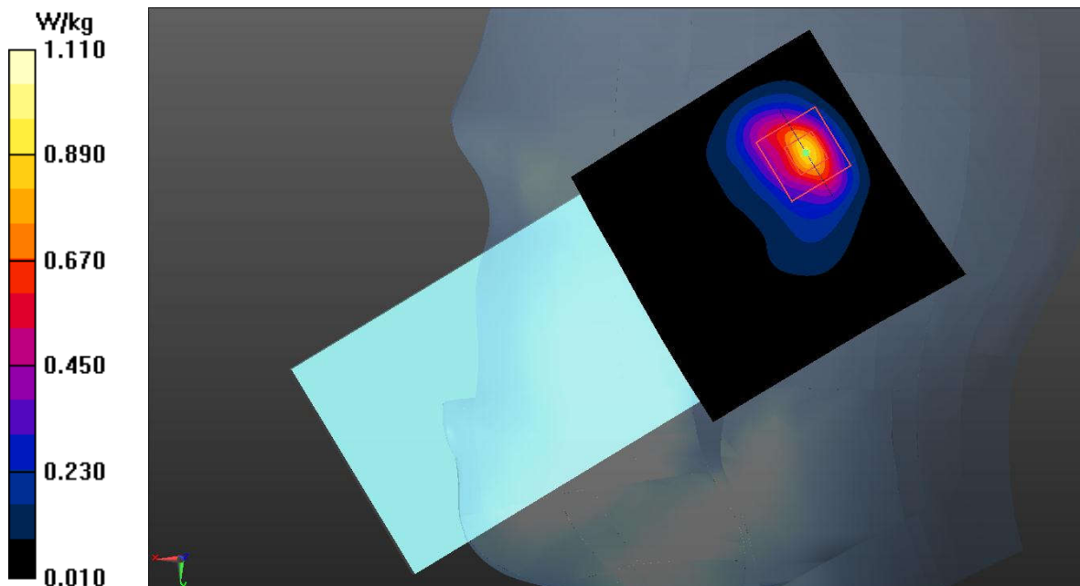
Fig.4 GSM 1900
