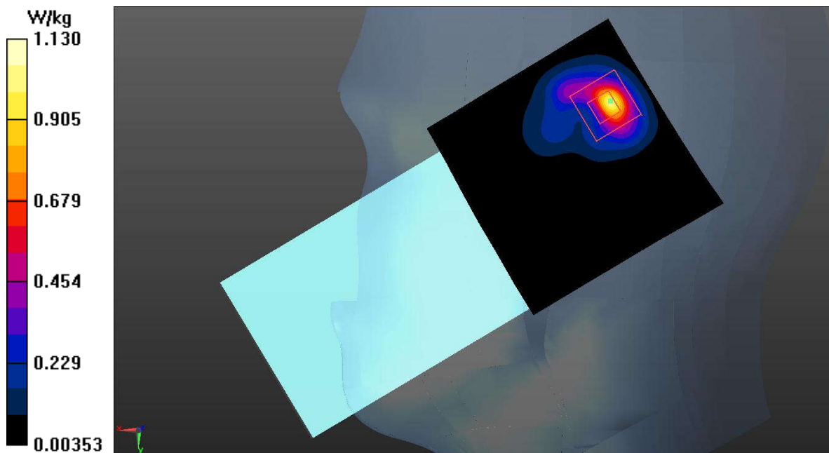
Fig.25 LTE Band 7
