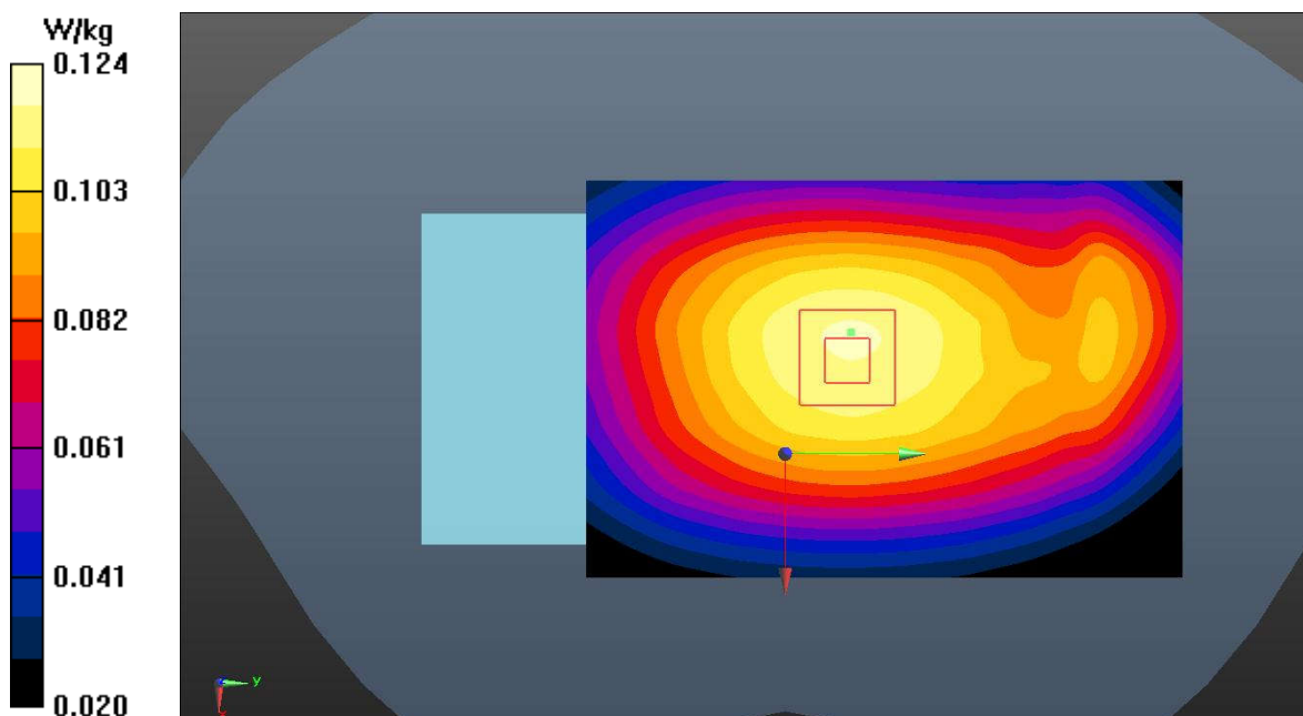
Fig.30 LTE Band 12
