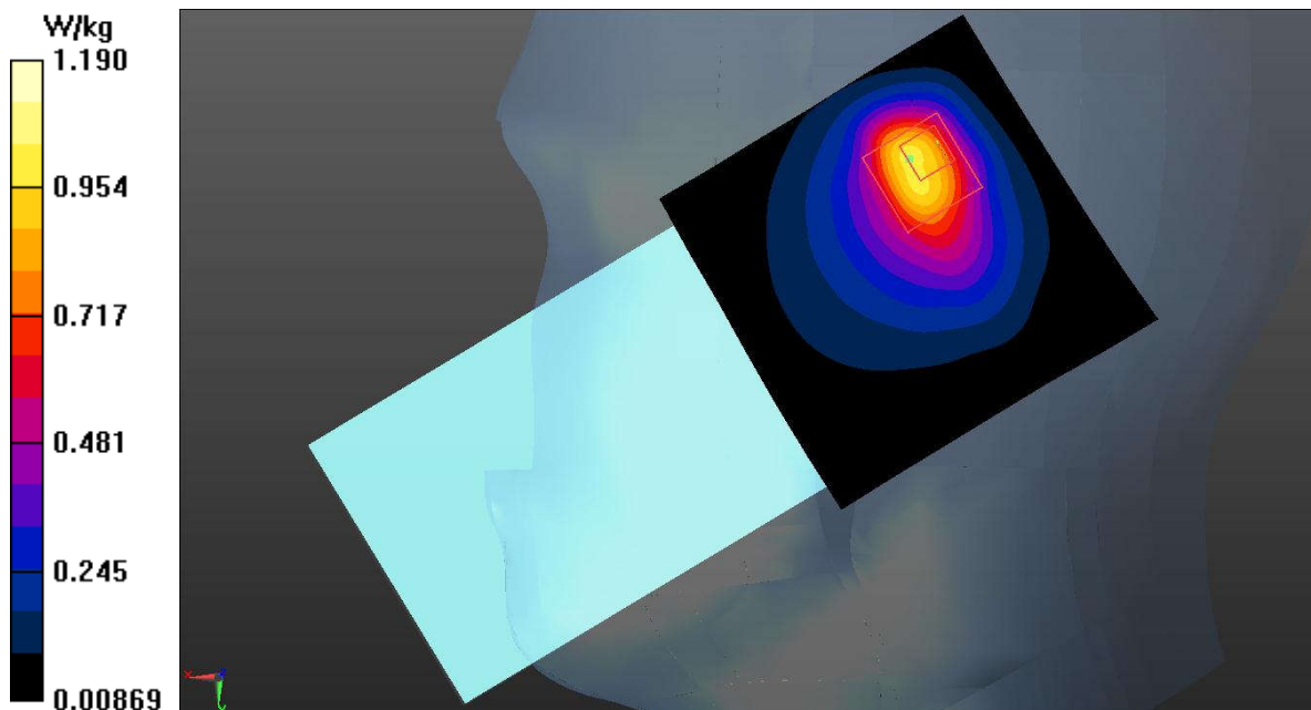
Fig.13 WCDMA Band 5
