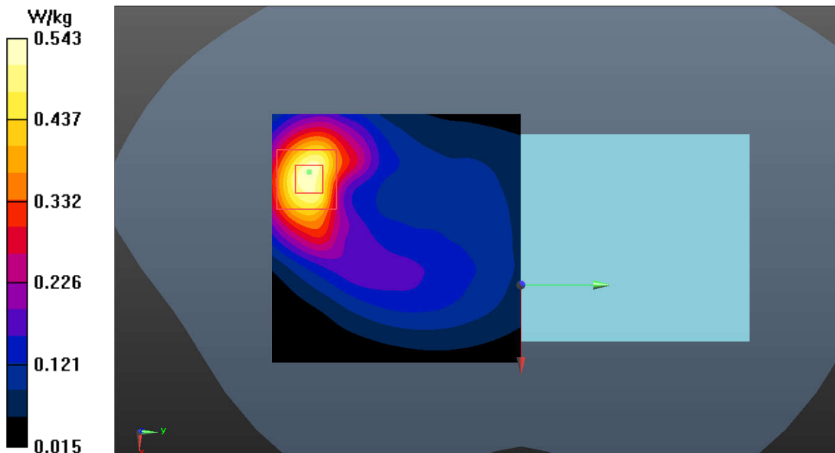
Fig.12 WCDMA Band 4
