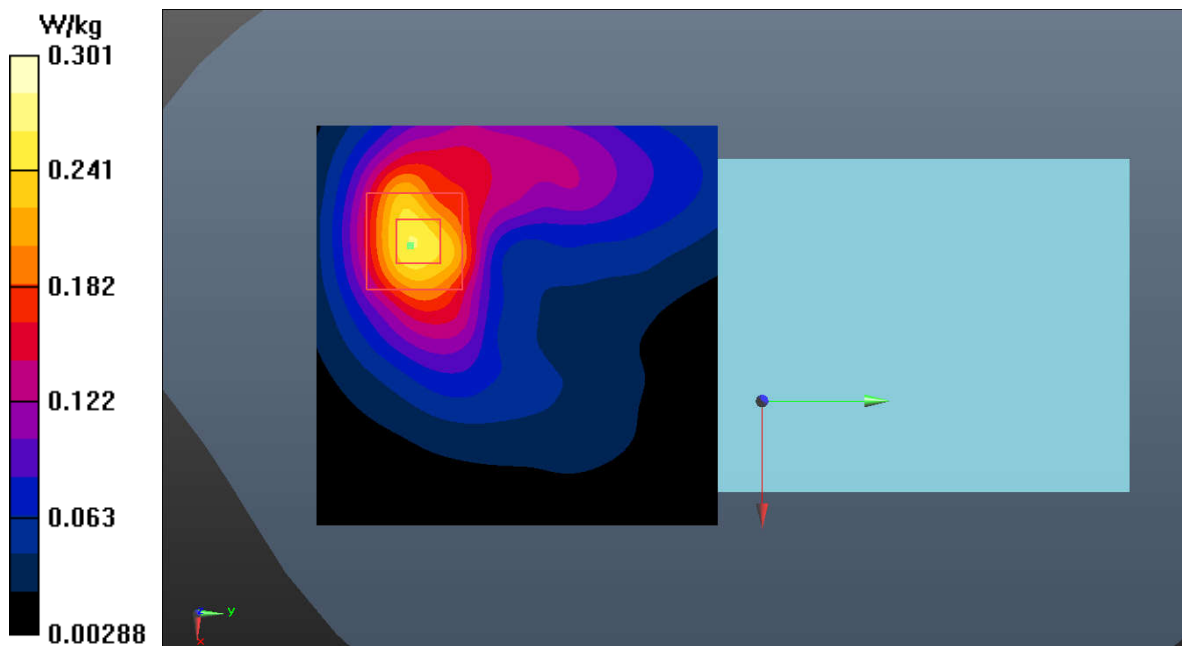
Fig.27 LTE Band 7
