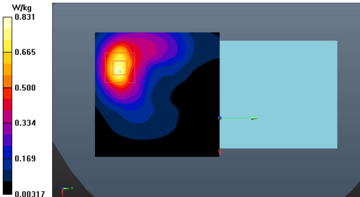
Fig.38 LTE Band 41
