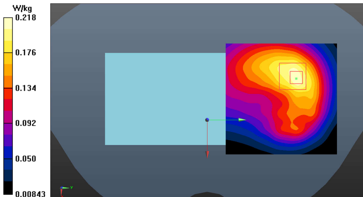
Fig.9 WCDMA Band 2
