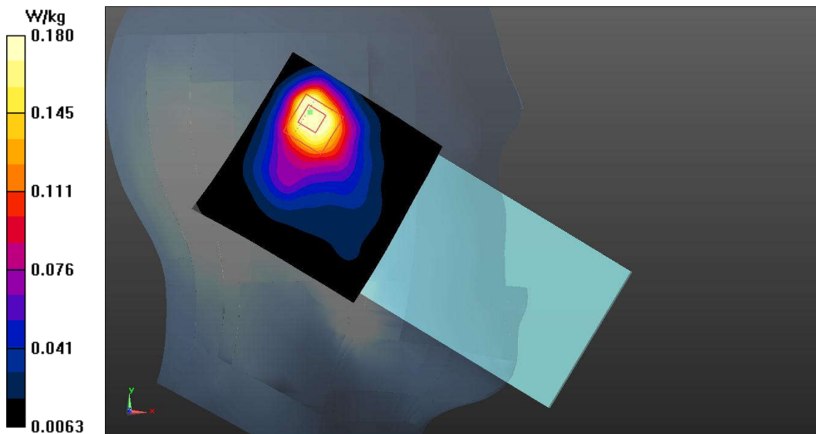
Fig.43 Bluetooth
