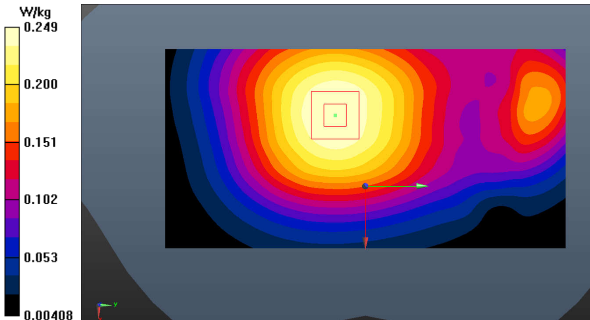
Fig.15 WCDMA Band 5
