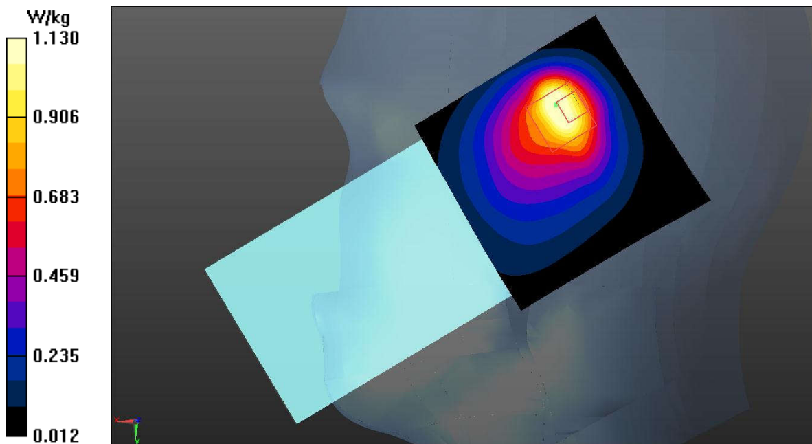
Fig.31 LTE Band 26
