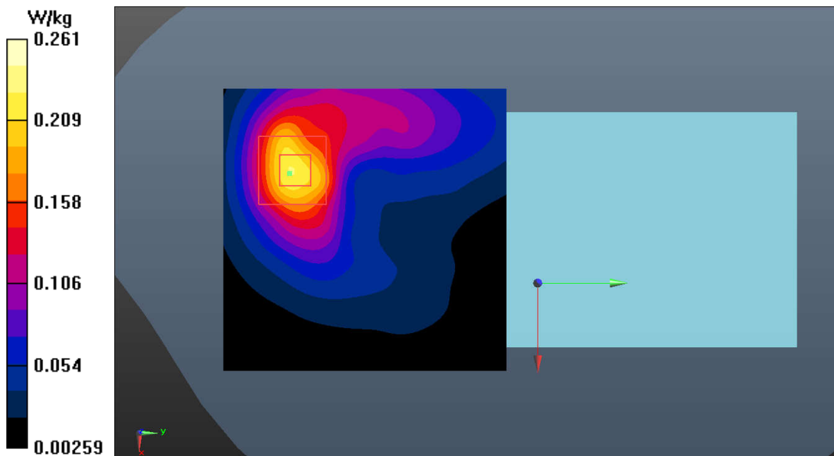
Fig.39 LTE Band 41
