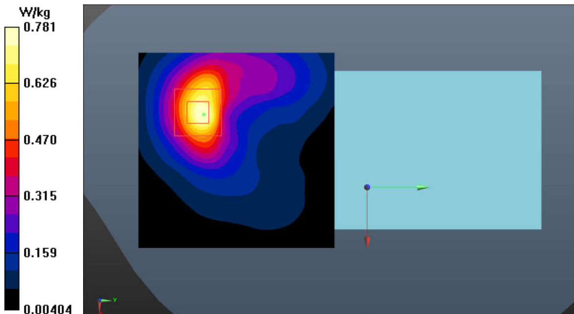
Fig.35 LTE Band 38
