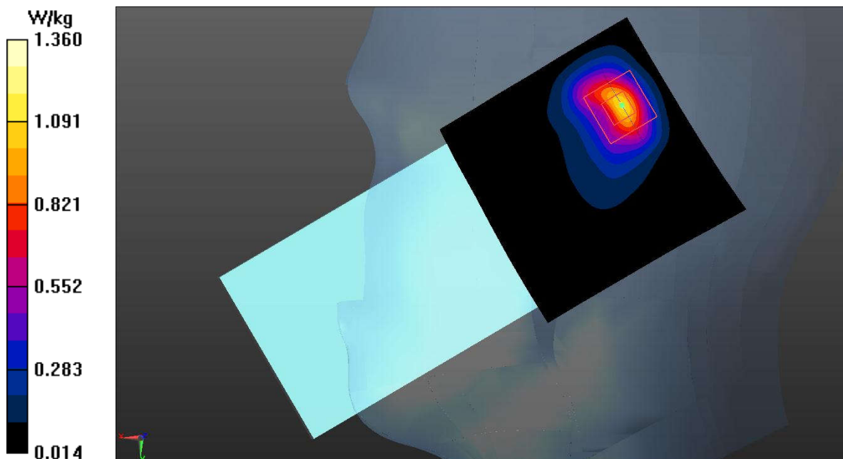
Fig.10 WCDMA Band 4
