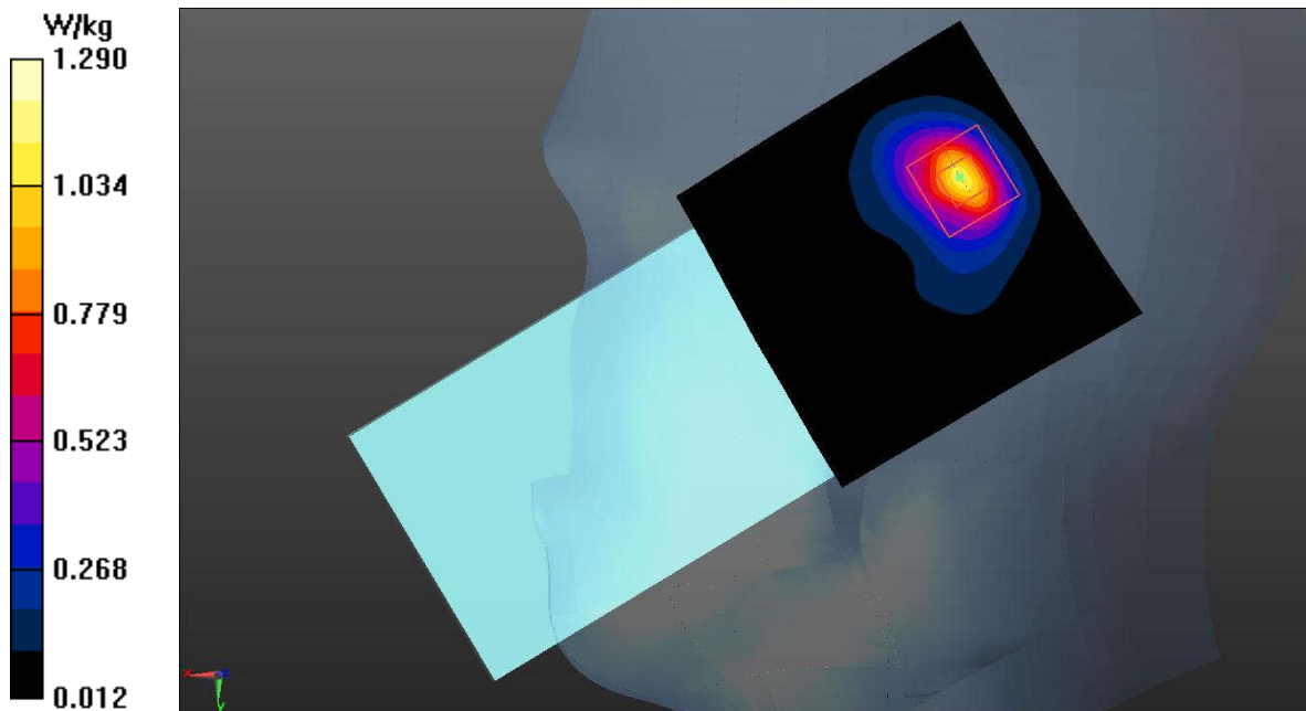
Fig.16 LTE Band 2
