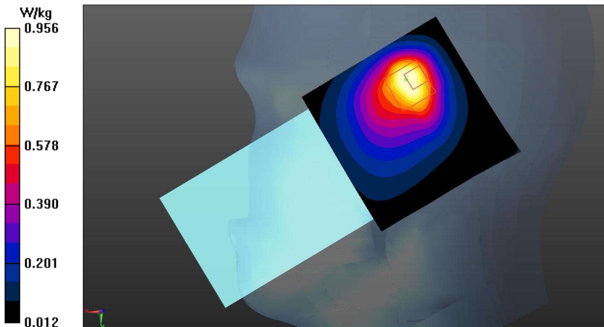
Fig.22 LTE Band 5
