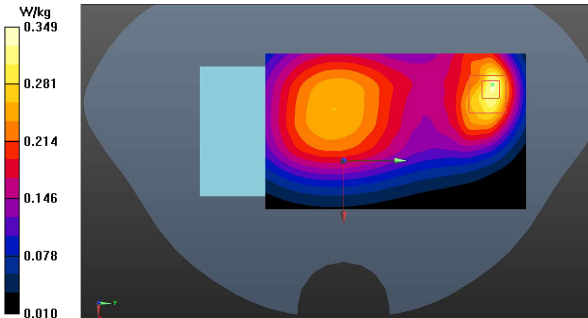
Fig.14 WCDMA Band 5
