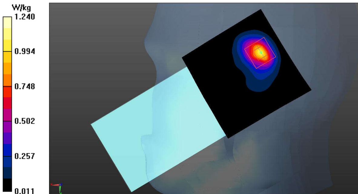
Fig.40 LTE Band 66
