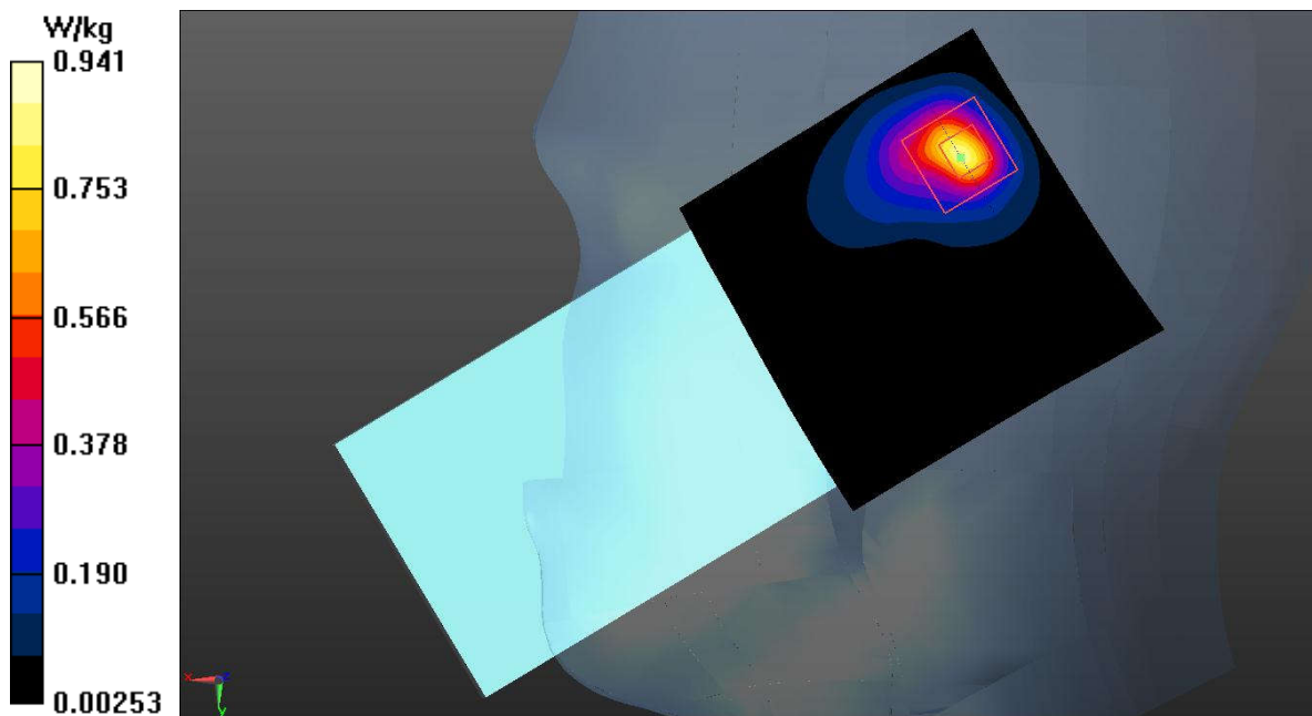
Fig.37 LTE Band 41
