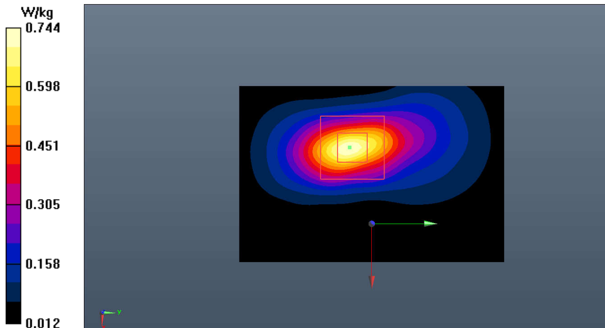
Fig.11 WCDMA Band 4
